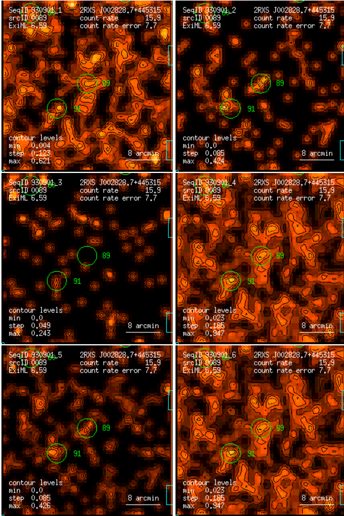
Figure 89: RASS 930901: detection 0089: band rate images, Gaussian filter: (1) PSPC channels 11 – 41, (2) 52 – 90, (3) 91 – 201, (4) 11 – 235, (5) 52 – 201, (6) 11 – 201. Broad band rates in counts/ks. Band rate contour levels in counts/ks/arcmin 2 .
