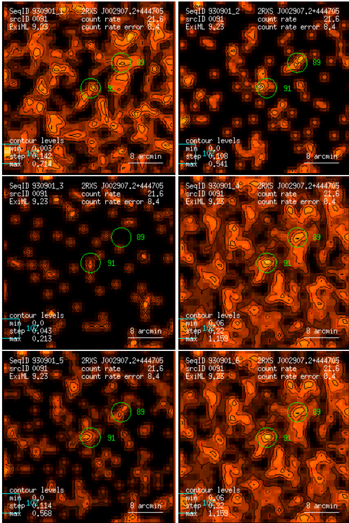
Figure 91: RASS 930901: detection 0091: band rate images, Gaussian filter: (1) PSPC channels 11 – 41, (2) 52 – 90, (3) 91 – 201, (4) 11 – 235, (5) 52 – 201, (6) 11 – 201. Broad band rates in counts/ks. Band rate contour levels in counts/ks/arcmin 2 .
