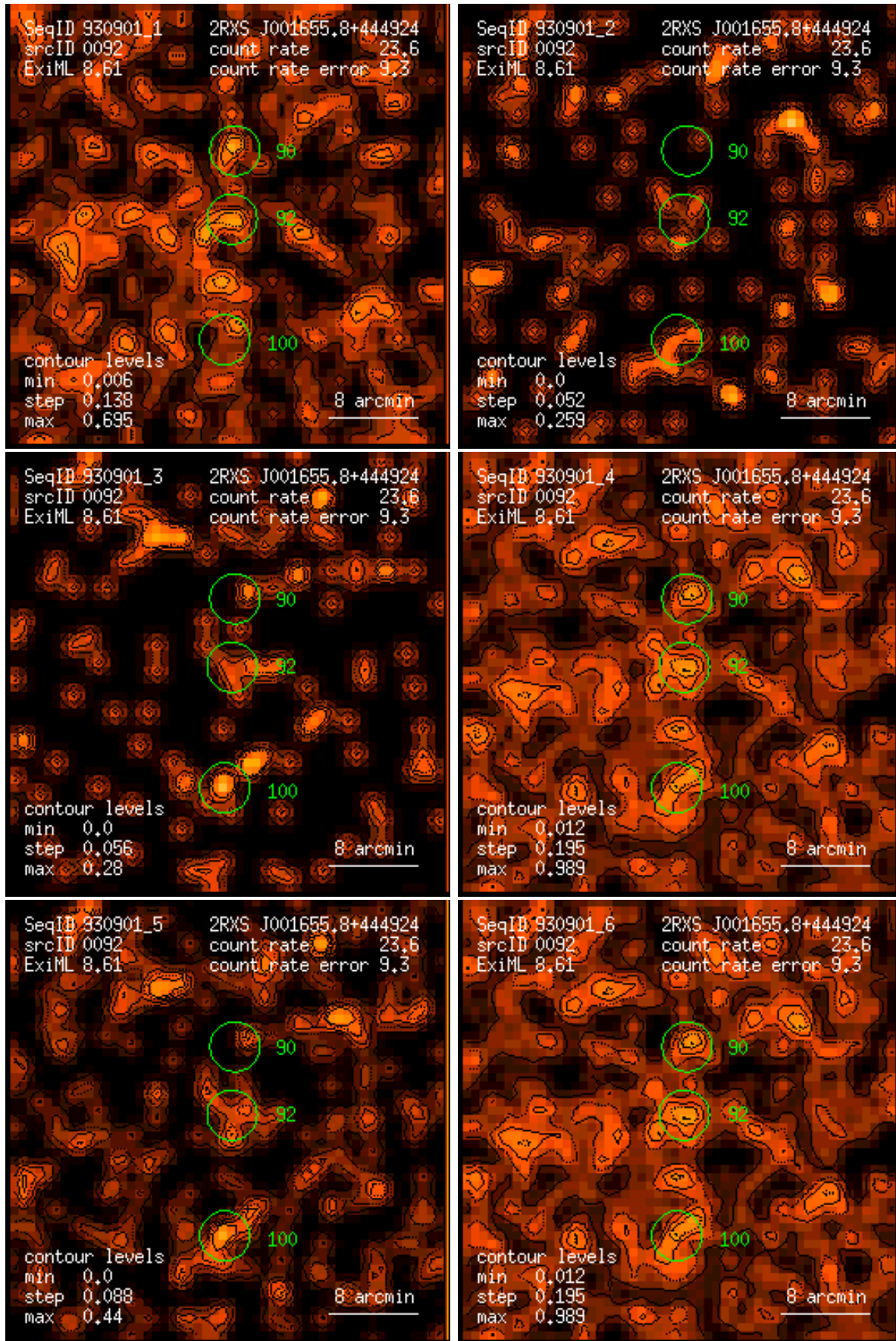
Figure 92: RASS 930901: detection 0092: band rate images, Gaussian filter: (1) PSPC channels 11 – 41, (2) 52 – 90, (3) 91 – 201, (4) 11 – 235, (5) 52 – 201, (6) 11 – 201. Broad band rates in counts/ks. Band rate contour levels in counts/ks/arcmin 2 .
