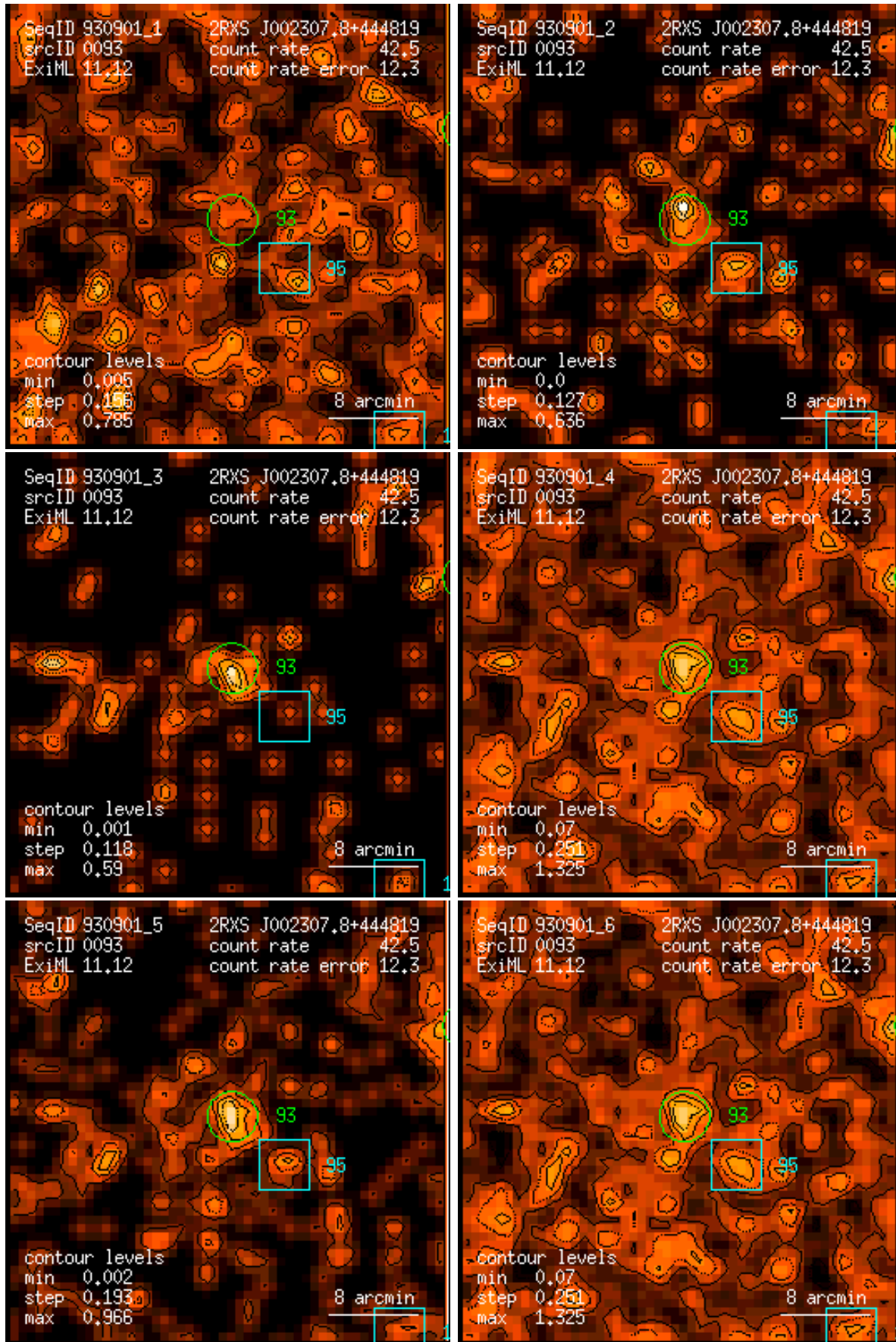
Figure 93: RASS 930901: detection 0093: band rate images, Gaussian filter: (1) PSPC channels 11 – 41, (2) 52 – 90, (3) 91 – 201, (4) 11 – 235, (5) 52 – 201, (6) 11 – 201. Broad band rates in counts/ks. Band rate contour levels in counts/ks/arcmin 2 .
