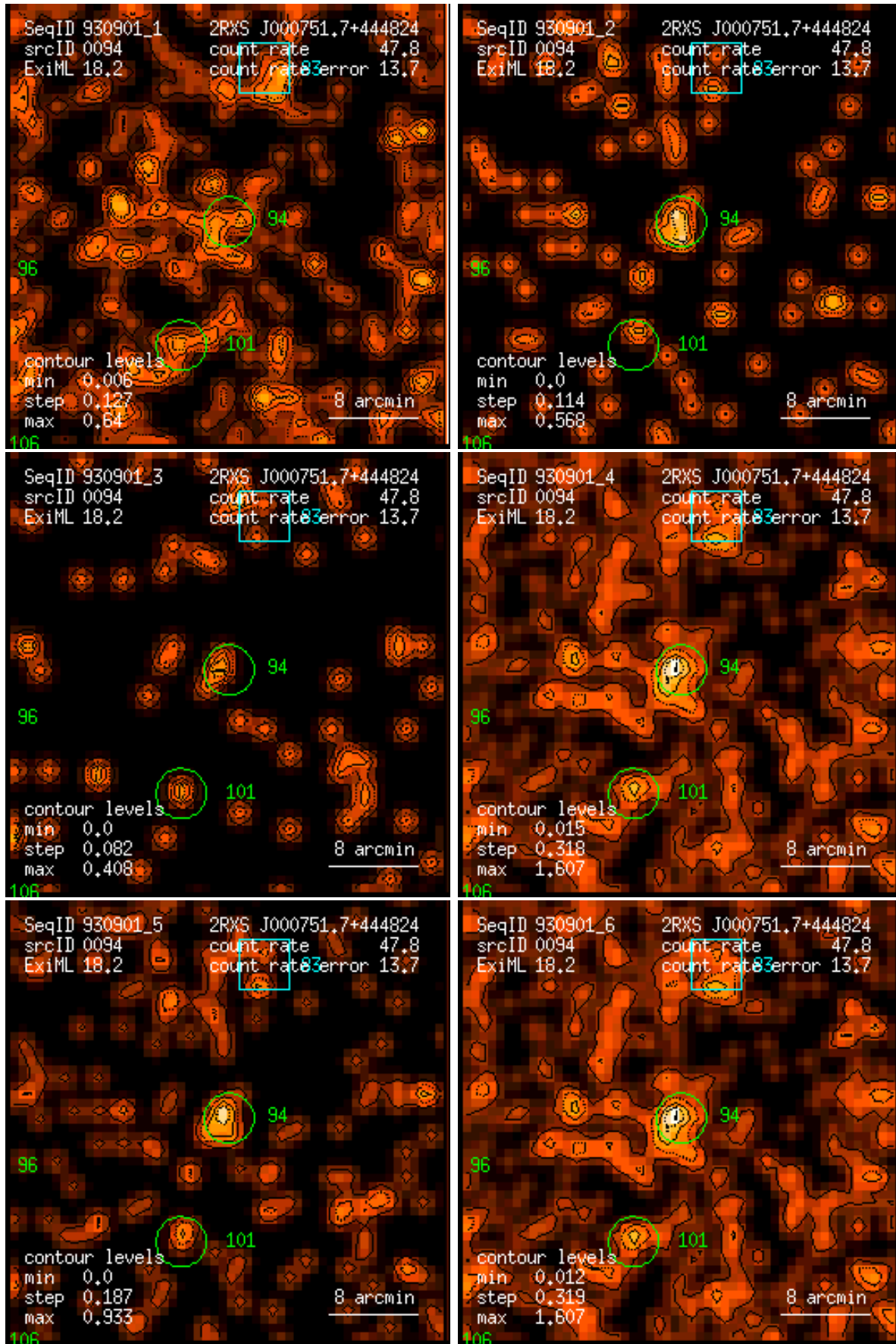
Figure 94: RASS 930901: detection 0094: band rate images, Gaussian filter: (1) PSPC channels 11 – 41, (2) 52 – 90, (3) 91 – 201, (4) 11 – 235, (5) 52 – 201, (6) 11 – 201. Broad band rates in counts/ks. Band rate contour levels in counts/ks/arcmin 2 .
