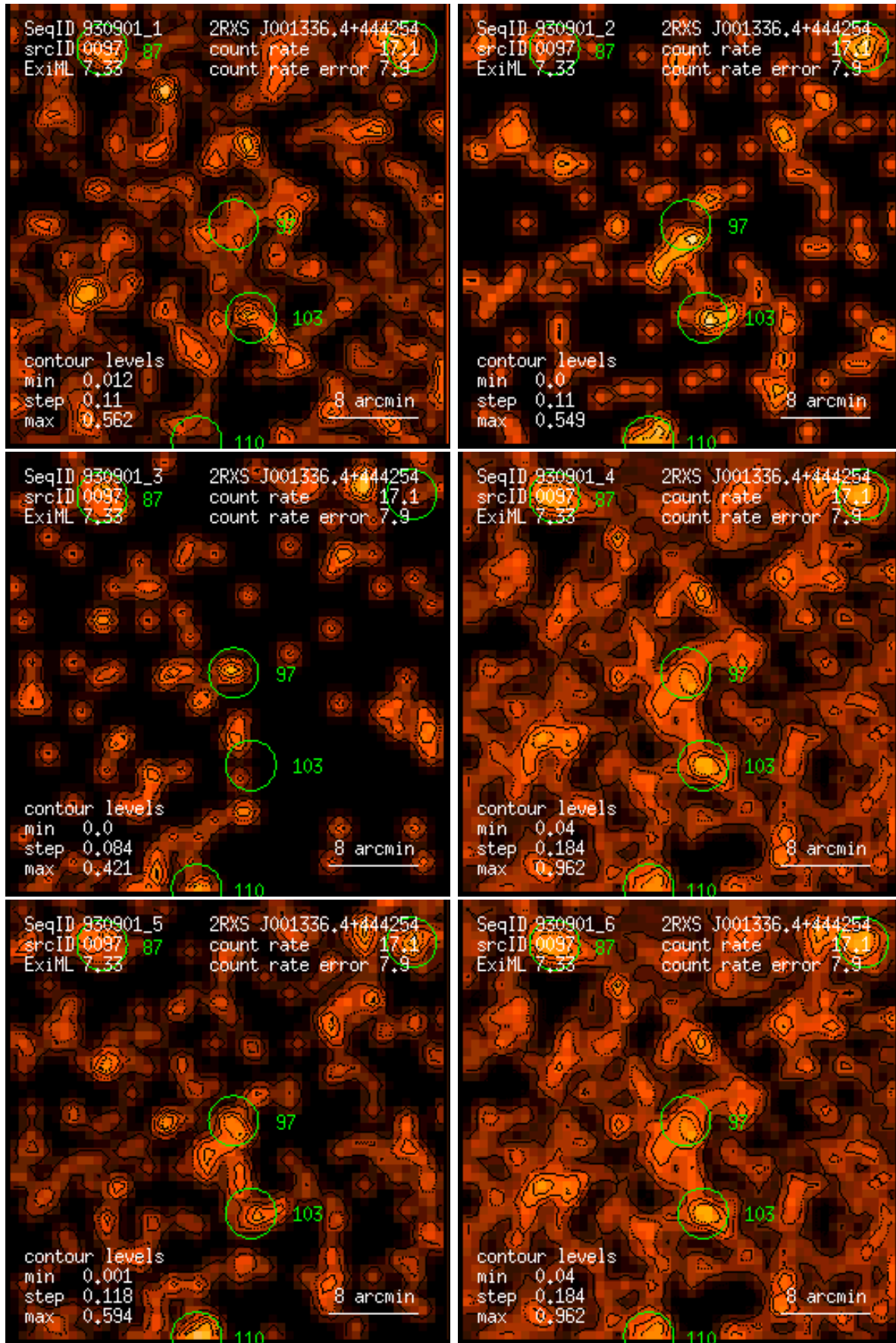
Figure 97: RASS 930901: detection 0097: band rate images, Gaussian filter: (1) PSPC channels 11 – 41, (2) 52 – 90, (3) 91 – 201, (4) 11 – 235, (5) 52 – 201, (6) 11 – 201. Broad band rates in counts/ks. Band rate contour levels in counts/ks/arcmin 2 .
