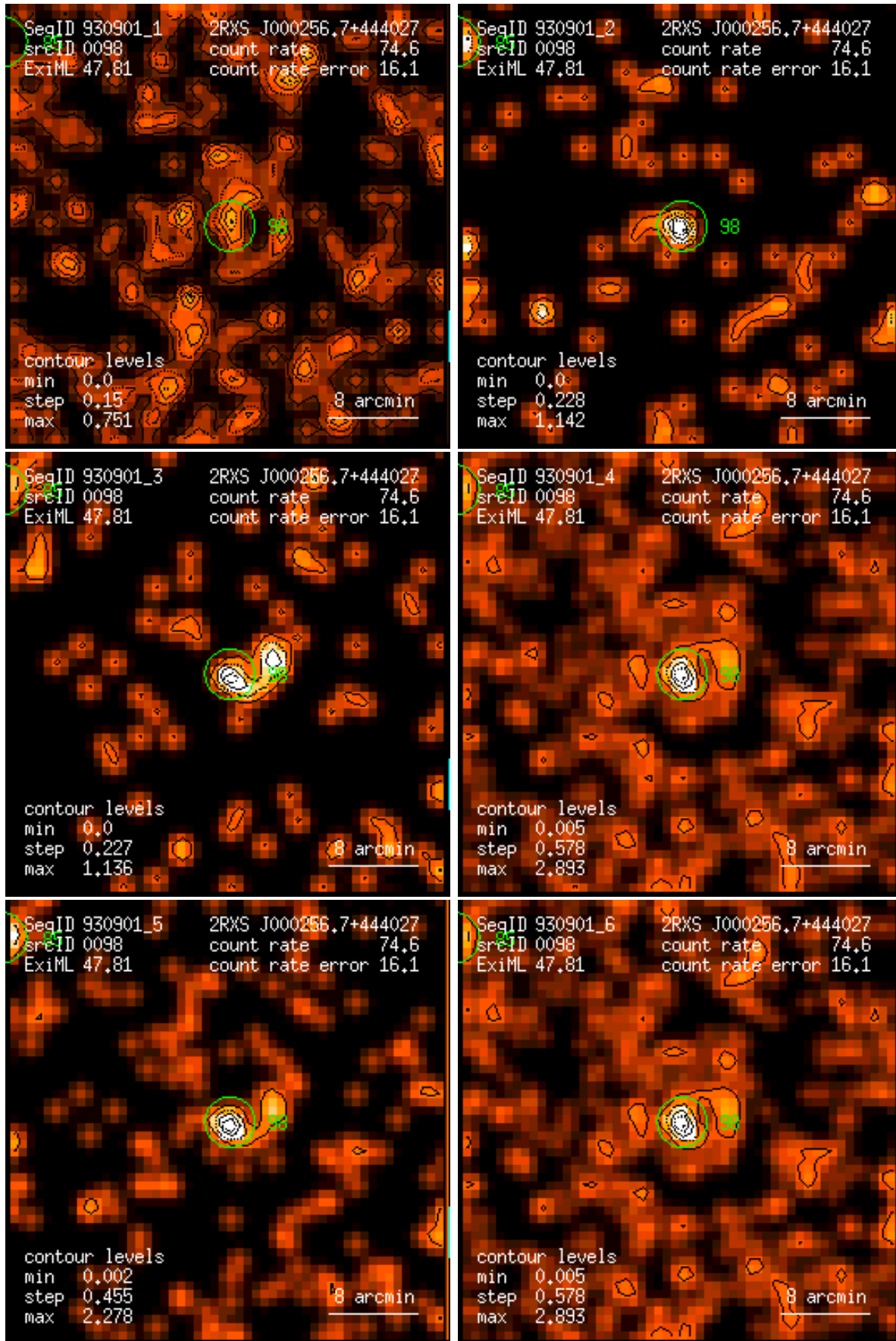
Figure 98: RASS 930901: detection 0098: band rate images, Gaussian filter: (1) PSPC channels 11 – 41, (2) 52 – 90, (3) 91 – 201, (4) 11 – 235, (5) 52 – 201, (6) 11 – 201. Broad band rates in counts/ks. Band rate contour levels in counts/ks/arcmin 2 .
