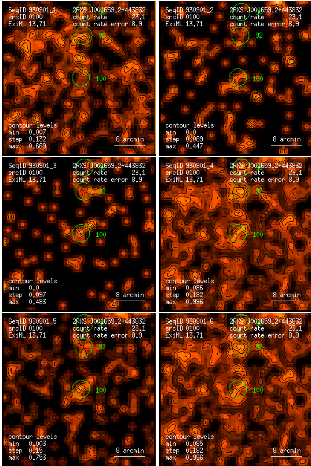
Figure 100: RASS 930901: detection 0100: band rate images, Gaussian filter: (1) PSPC channels 11 – 41, (2) 52 – 90, (3) 91 – 201, (4) 11 – 235, (5) 52 – 201, (6) 11 – 201. Broad band rates in counts/ks. Band rate contour levels in counts/ks/arcmin 2 .
