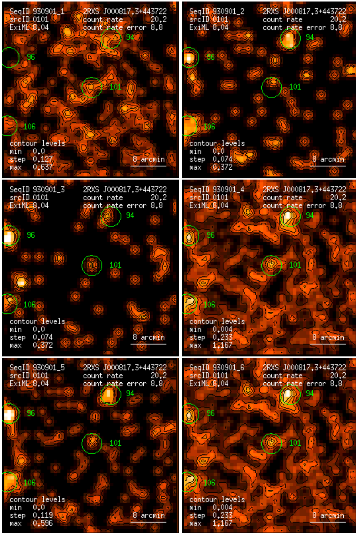
Figure 101: RASS 930901: detection 0101: band rate images, Gaussian filter: (1) PSPC channels 11 – 41, (2) 52 – 90, (3) 91 – 201, (4) 11 – 235, (5) 52 – 201, (6) 11 – 201. Broad band rates in counts/ks. Band rate contour levels in counts/ks/arcmin 2 .
