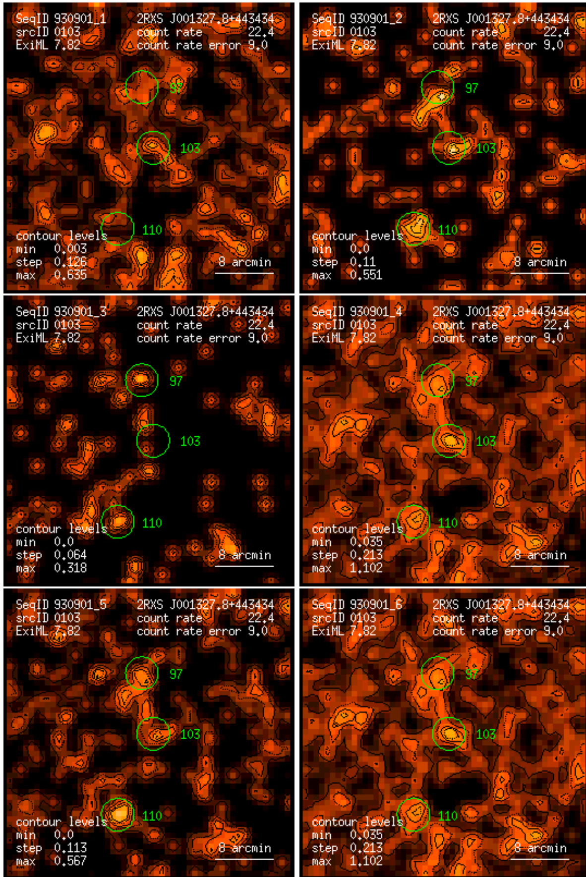
Figure 103: RASS 930901: detection 0103: band rate images, Gaussian filter: (1) PSPC channels 11 – 41, (2) 52 – 90, (3) 91 – 201, (4) 11 – 235, (5) 52 – 201, (6) 11 – 201. Broad band rates in counts/ks. Band rate contour levels in counts/ks/arcmin 2 .
