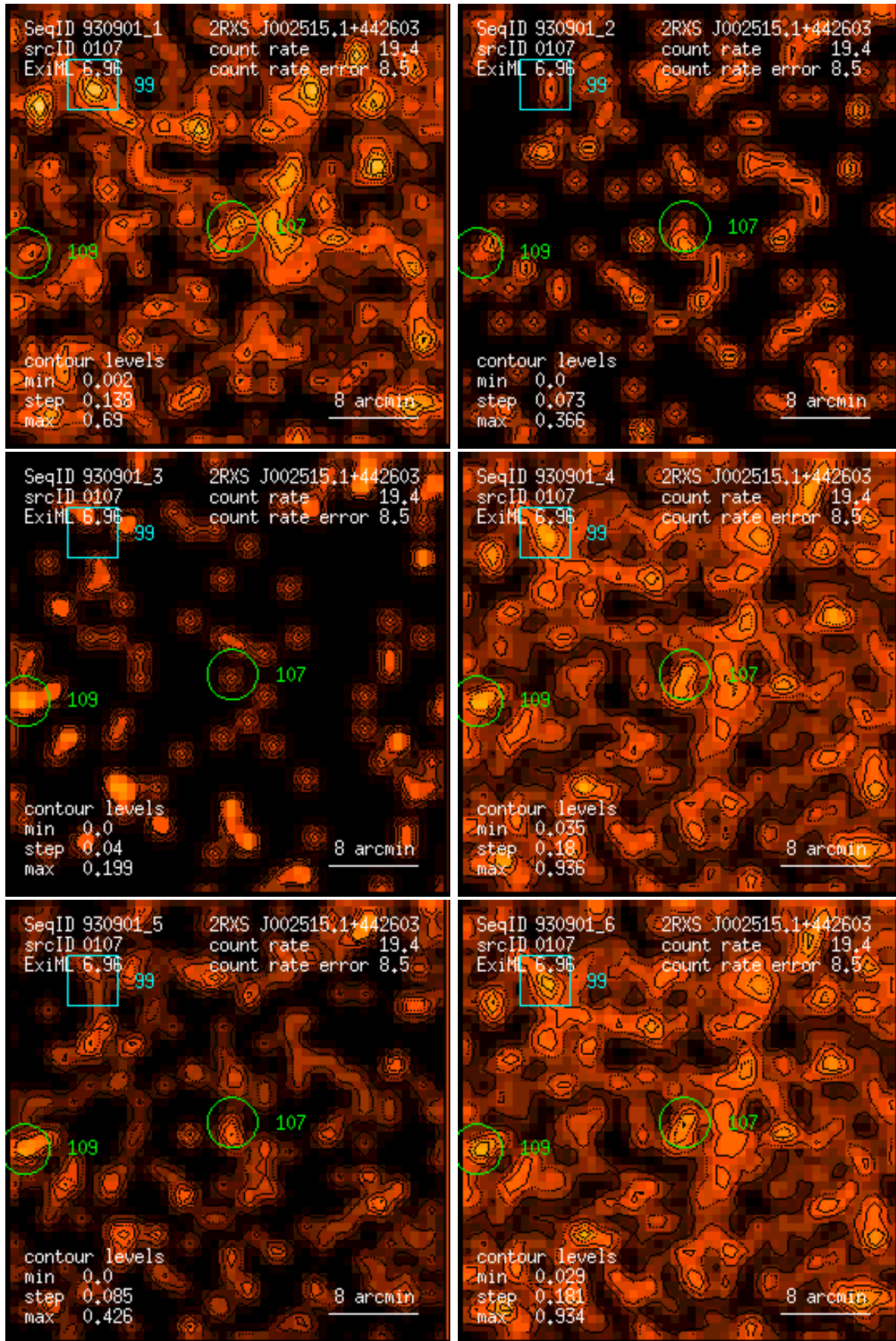
Figure 107: RASS 930901: detection 0107: band rate images, Gaussian filter: (1) PSPC channels 11 – 41, (2) 52 – 90, (3) 91 – 201, (4) 11 – 235, (5) 52 – 201, (6) 11 – 201. Broad band rates in counts/ks. Band rate contour levels in counts/ks/arcmin 2 .
