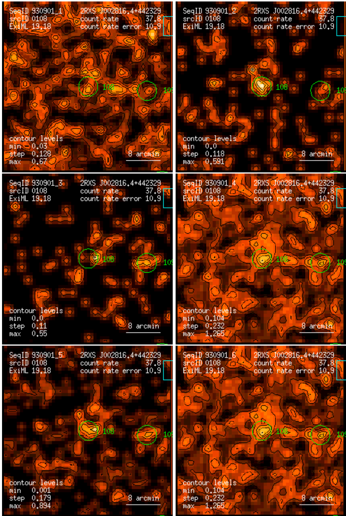
Figure 108: RASS 930901: detection 0108: band rate images, Gaussian filter: (1) PSPC channels 11 – 41, (2) 52 – 90, (3) 91 – 201, (4) 11 – 235, (5) 52 – 201, (6) 11 – 201. Broad band rates in counts/ks. Band rate contour levels in counts/ks/arcmin 2 .
