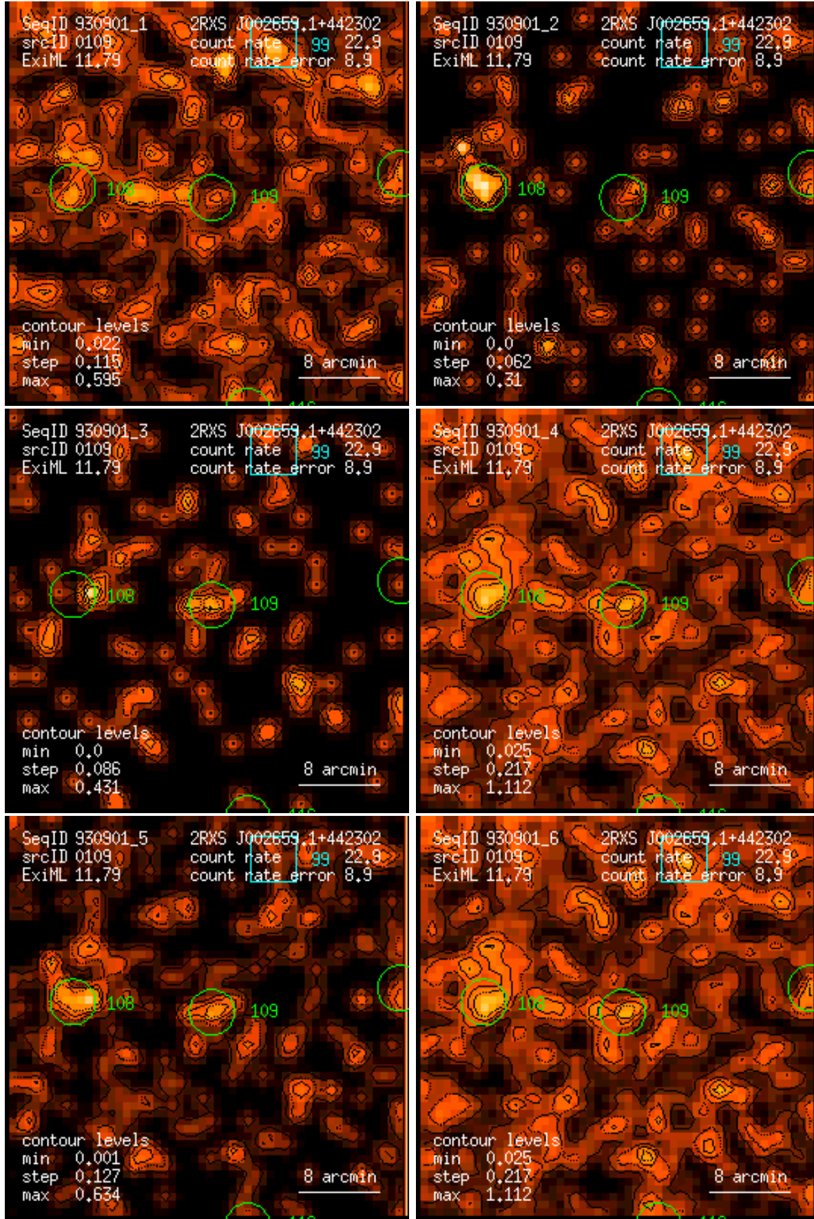
Figure 109: RASS 930901: detection 0109: band rate images, Gaussian filter: (1) PSPC channels 11 – 41, (2) 52 – 90, (3) 91 – 201, (4) 11 – 235, (5) 52 – 201, (6) 11 – 201. Broad band rates in counts/ks. Band rate contour levels in counts/ks/arcmin 2 .
