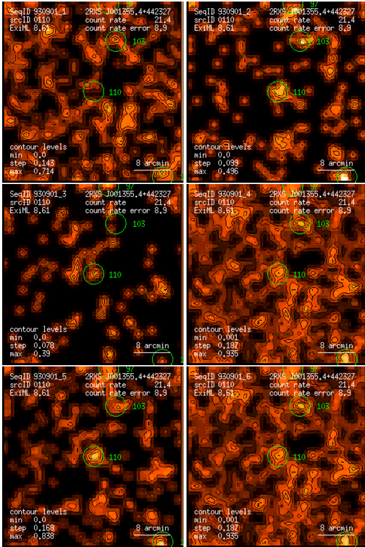
Figure 110: RASS 930901: detection 0110: band rate images, Gaussian filter: (1) PSPC channels 11 – 41, (2) 52 – 90, (3) 91 – 201, (4) 11 – 235, (5) 52 – 201, (6) 11 – 201. Broad band rates in counts/ks. Band rate contour levels in counts/ks/arcmin 2 .
