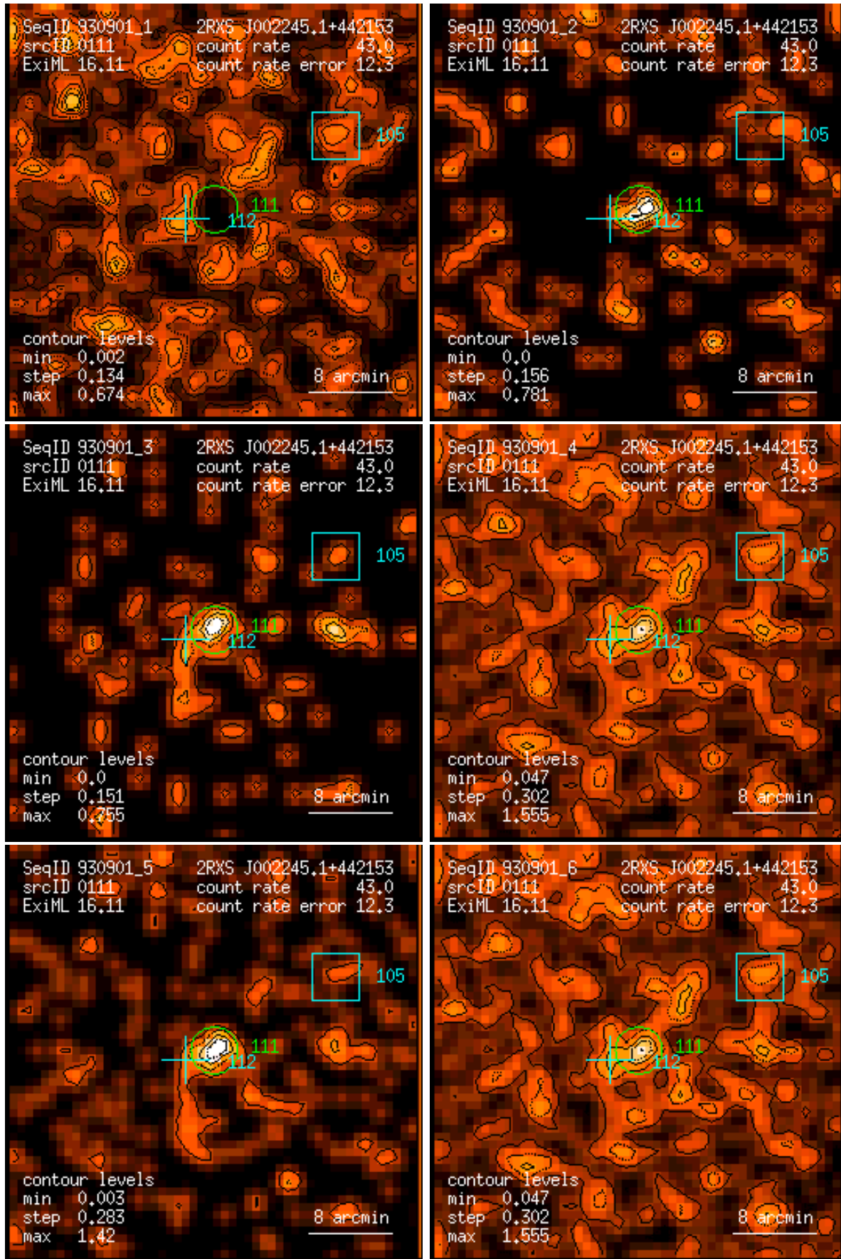
Figure 111: RASS 930901: detection 0111: band rate images, Gaussian filter: (1) PSPC channels 11 – 41, (2) 52 – 90, (3) 91 – 201, (4) 11 – 235, (5) 52 – 201, (6) 11 – 201. Broad band rates in counts/ks. Band rate contour levels in counts/ks/arcmin 2 .
