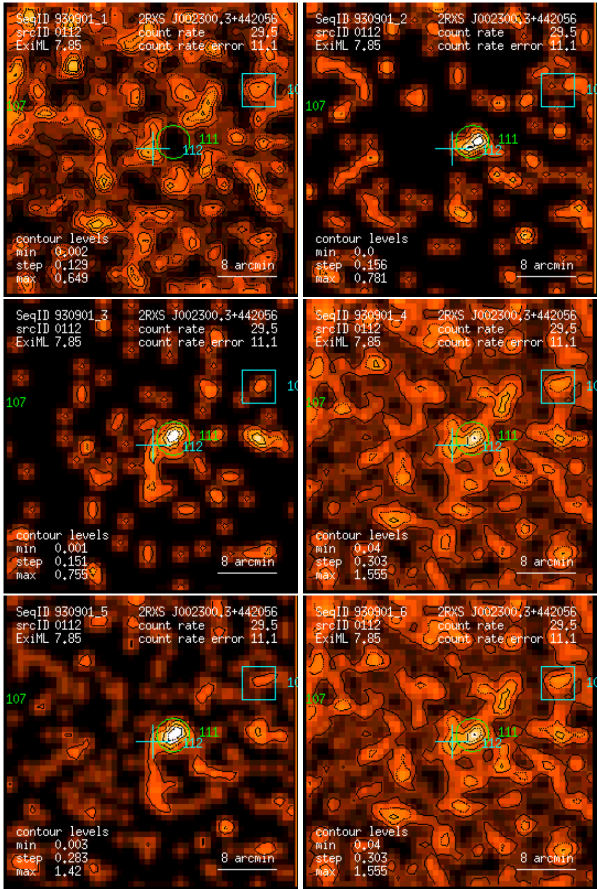
Figure 112: RASS 930901: detection 0112: band rate images, Gaussian filter: (1) PSPC channels 11 – 41, (2) 52 – 90, (3) 91 – 201, (4) 11 – 235, (5) 52 – 201, (6) 11 – 201. Broad band rates in counts/ks. Band rate contour levels in counts/ks/arcmin 2 .
