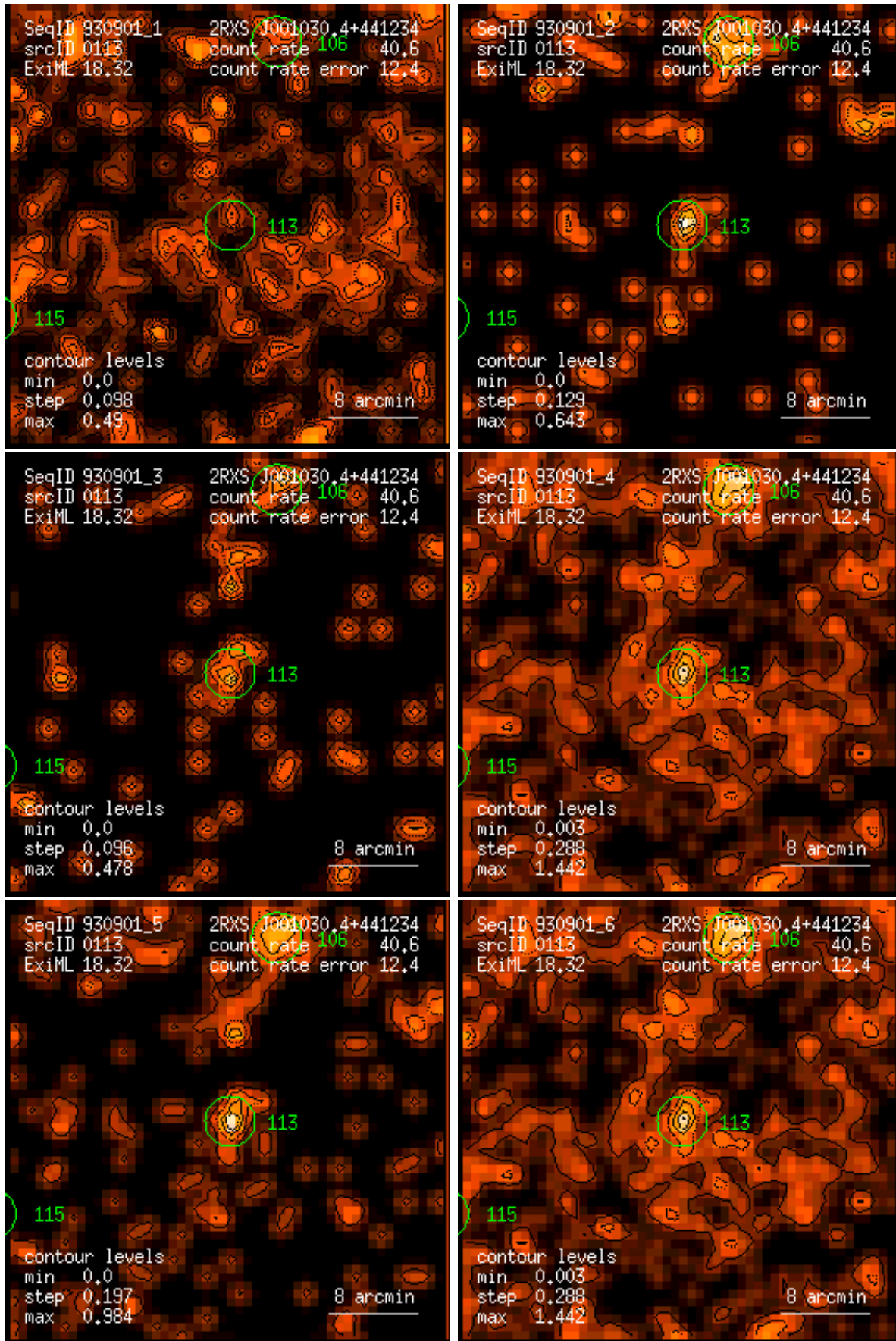
Figure 113: RASS 930901: detection 0113: band rate images, Gaussian filter: (1) PSPC channels 11 – 41, (2) 52 – 90, (3) 91 – 201, (4) 11 – 235, (5) 52 – 201, (6) 11 – 201. Broad band rates in counts/ks. Band rate contour levels in counts/ks/arcmin 2 .
