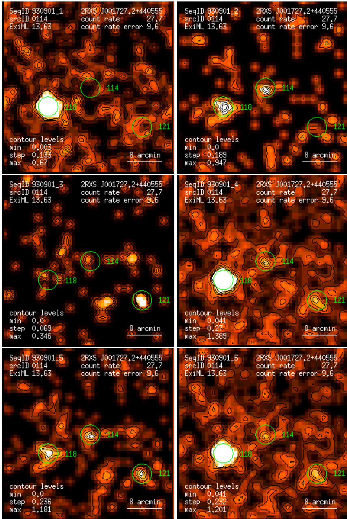
Figure 114: RASS 930901: detection 0114: band rate images, Gaussian filter: (1) PSPC channels 11 – 41, (2) 52 – 90, (3) 91 – 201, (4) 11 – 235, (5) 52 – 201, (6) 11 – 201. Broad band rates in counts/ks. Band rate contour levels in counts/ks/arcmin 2 .
