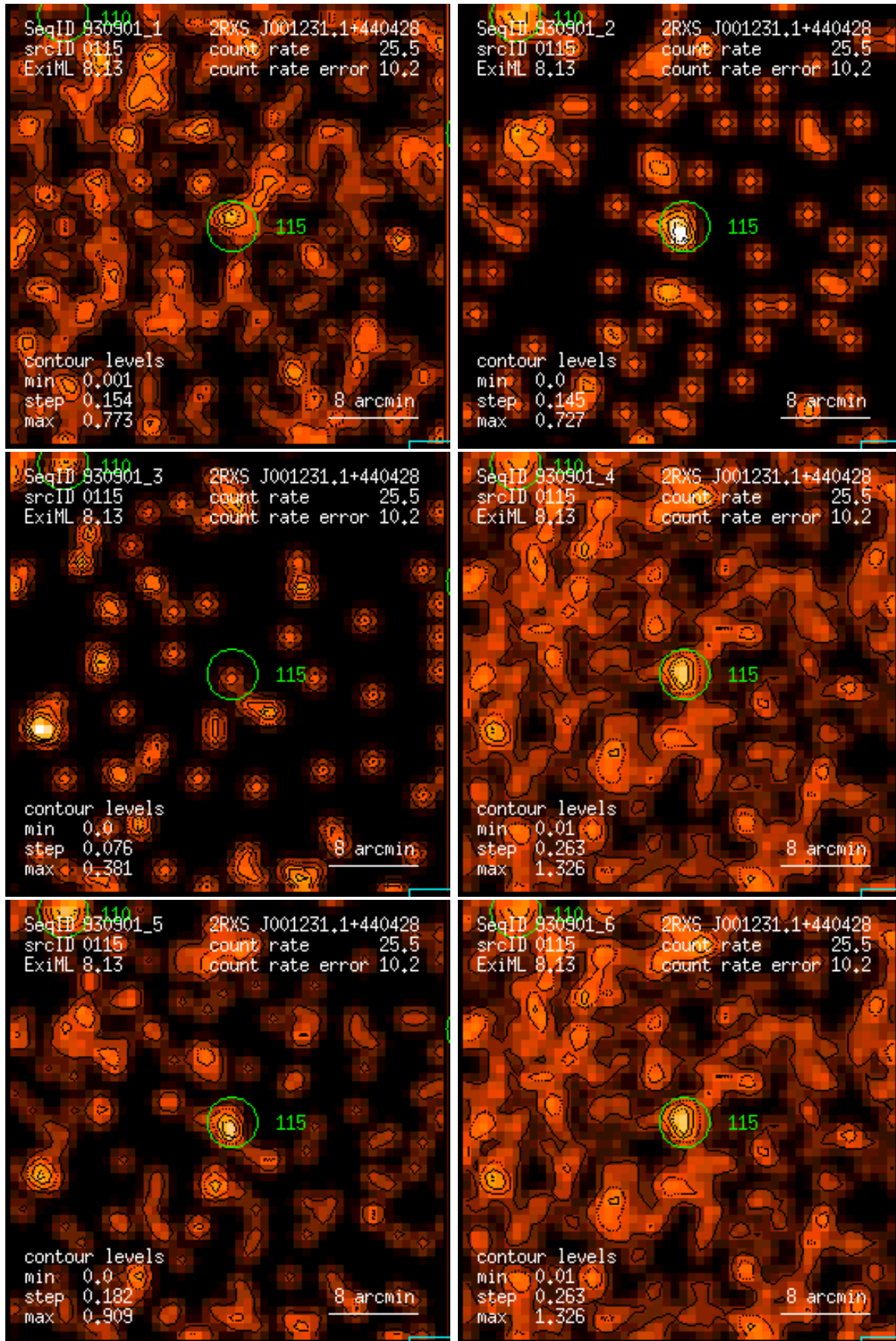
Figure 115: RASS 930901: detection 0115: band rate images, Gaussian filter: (1) PSPC channels 11 – 41, (2) 52 – 90, (3) 91 – 201, (4) 11 – 235, (5) 52 – 201, (6) 11 – 201. Broad band rates in counts/ks. Band rate contour levels in counts/ks/arcmin 2 .
