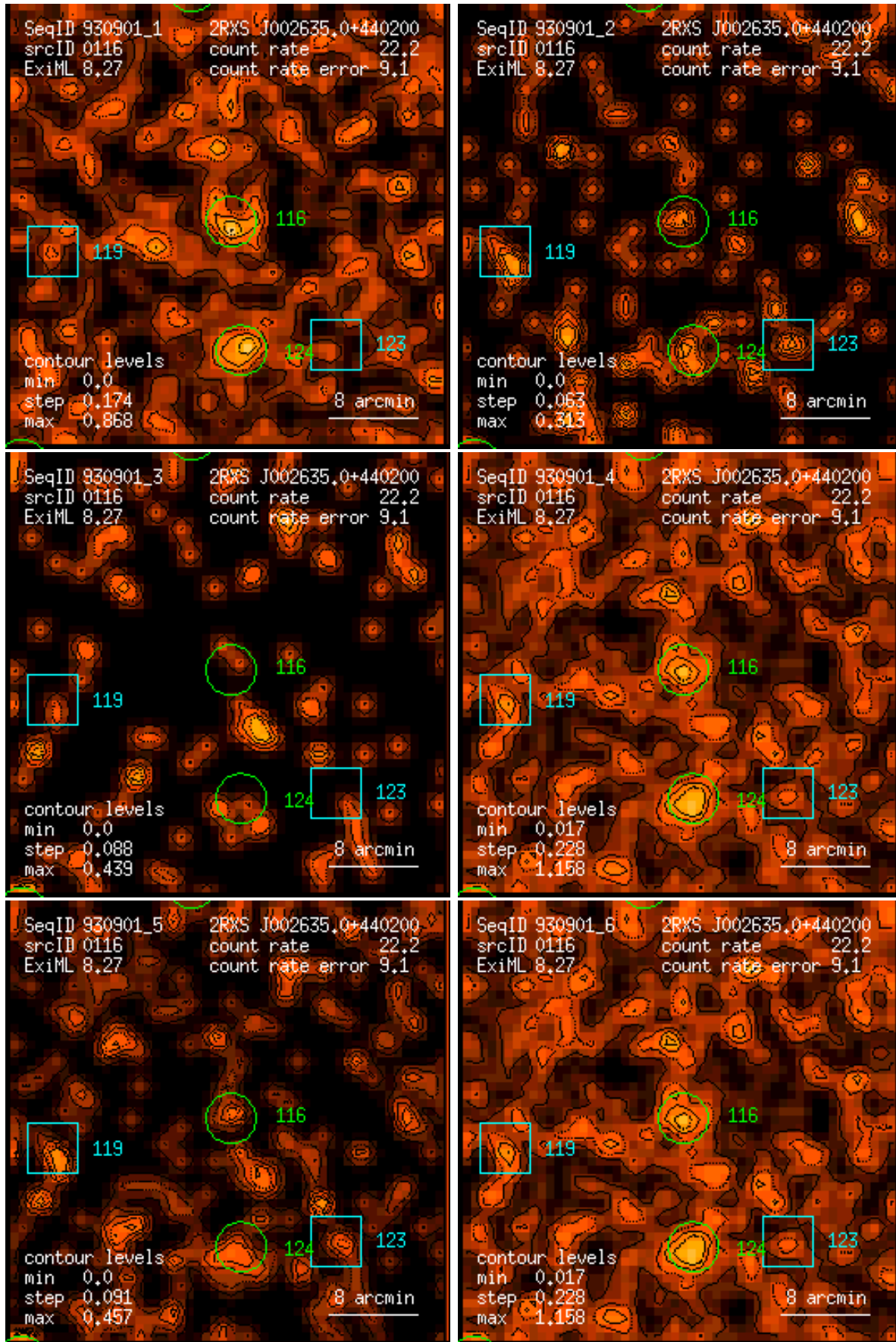
Figure 116: RASS 930901: detection 0116: band rate images, Gaussian filter: (1) PSPC channels 11 – 41, (2) 52 – 90, (3) 91 – 201, (4) 11 – 235, (5) 52 – 201, (6) 11 – 201. Broad band rates in counts/ks. Band rate contour levels in counts/ks/arcmin 2 .
