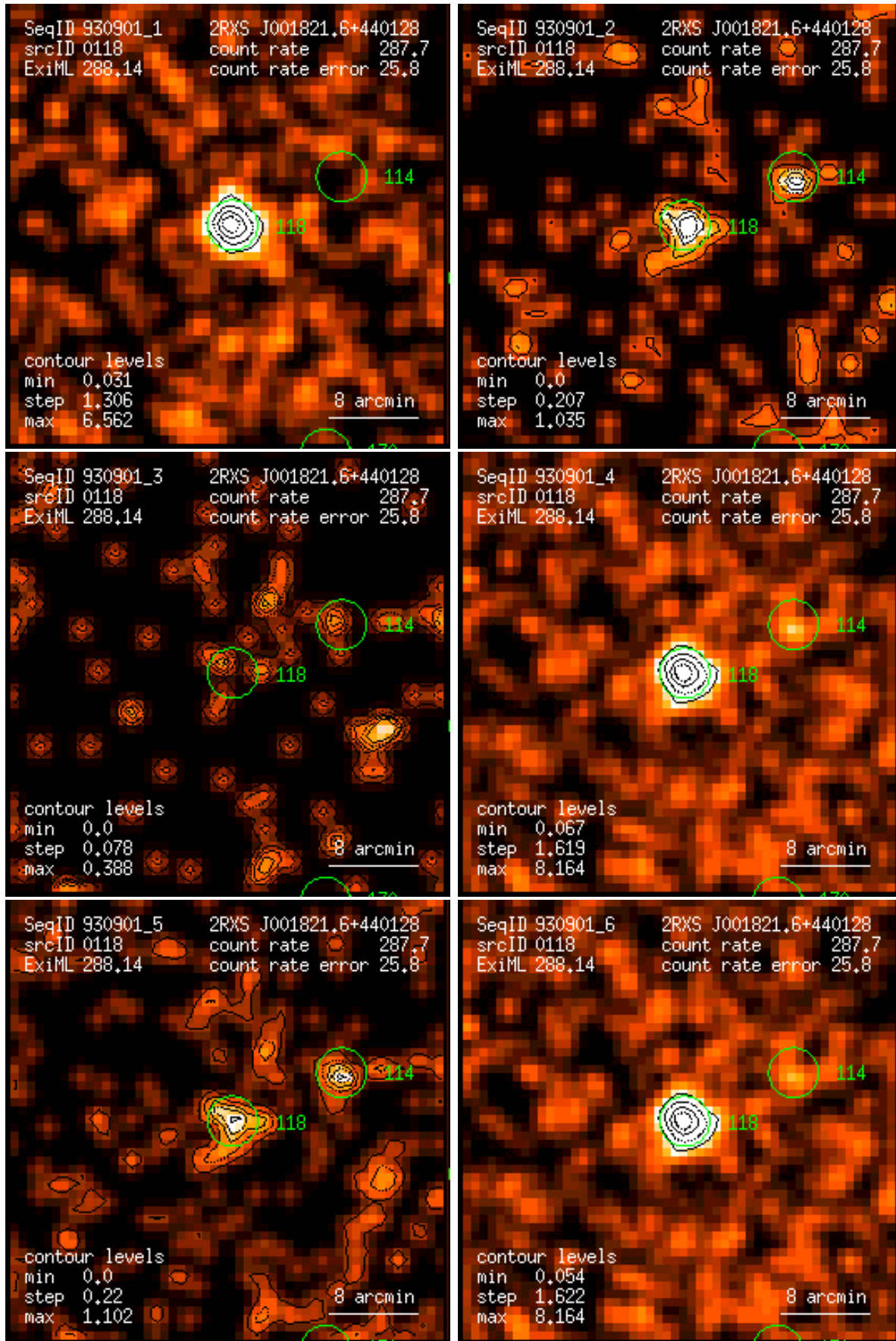
Figure 118: RASS 930901: detection 0118: band rate images, Gaussian filter: (1) PSPC channels 11 – 41, (2) 52 – 90, (3) 91 – 201, (4) 11 – 235, (5) 52 – 201, (6) 11 – 201. Broad band rates in counts/ks. Band rate contour levels in counts/ks/arcmin 2 .
