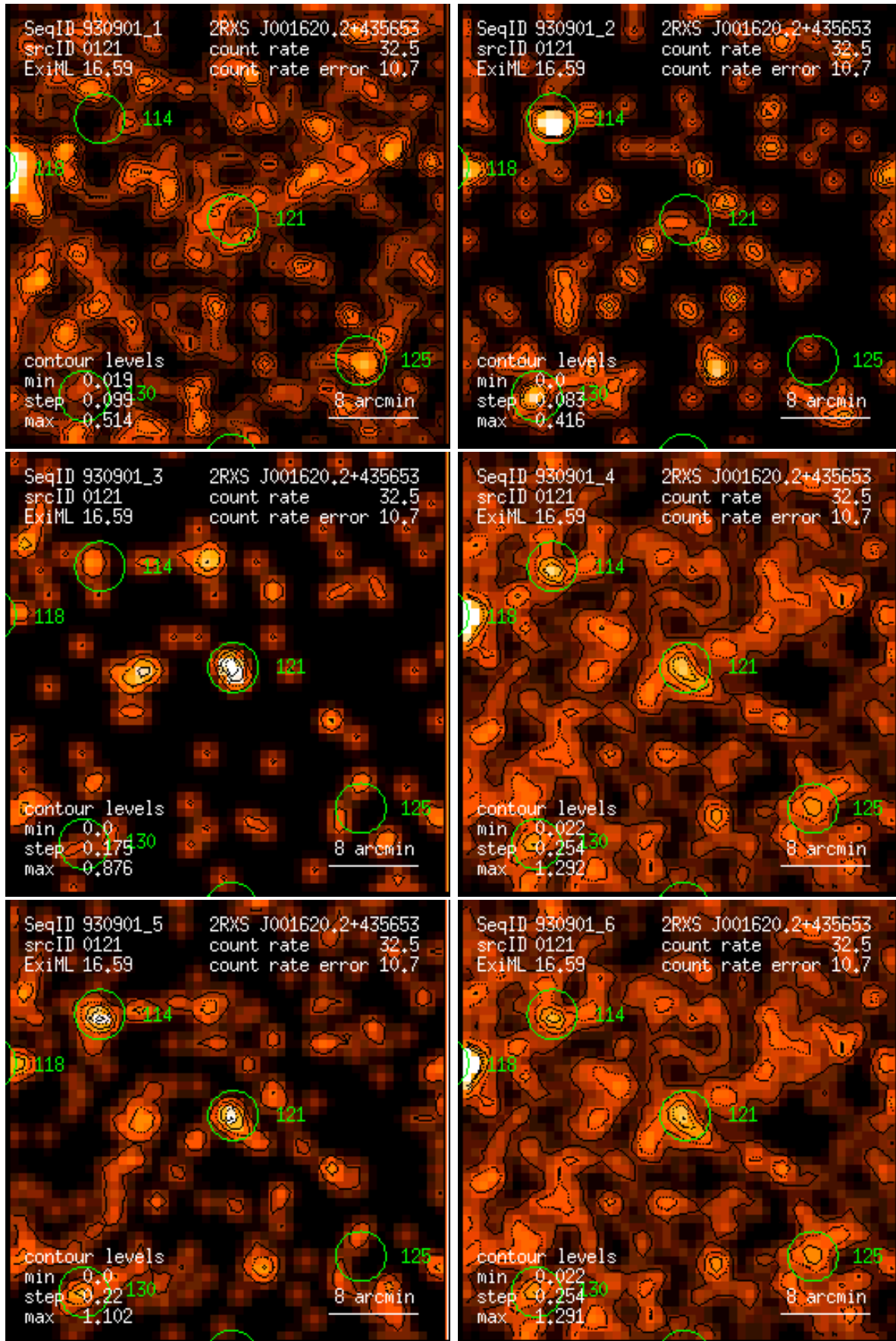
Figure 121: RASS 930901: detection 0121: band rate images, Gaussian filter: (1) PSPC channels 11 – 41, (2) 52 – 90, (3) 91 – 201, (4) 11 – 235, (5) 52 – 201, (6) 11 – 201. Broad band rates in counts/ks. Band rate contour levels in counts/ks/arcmin 2 .
