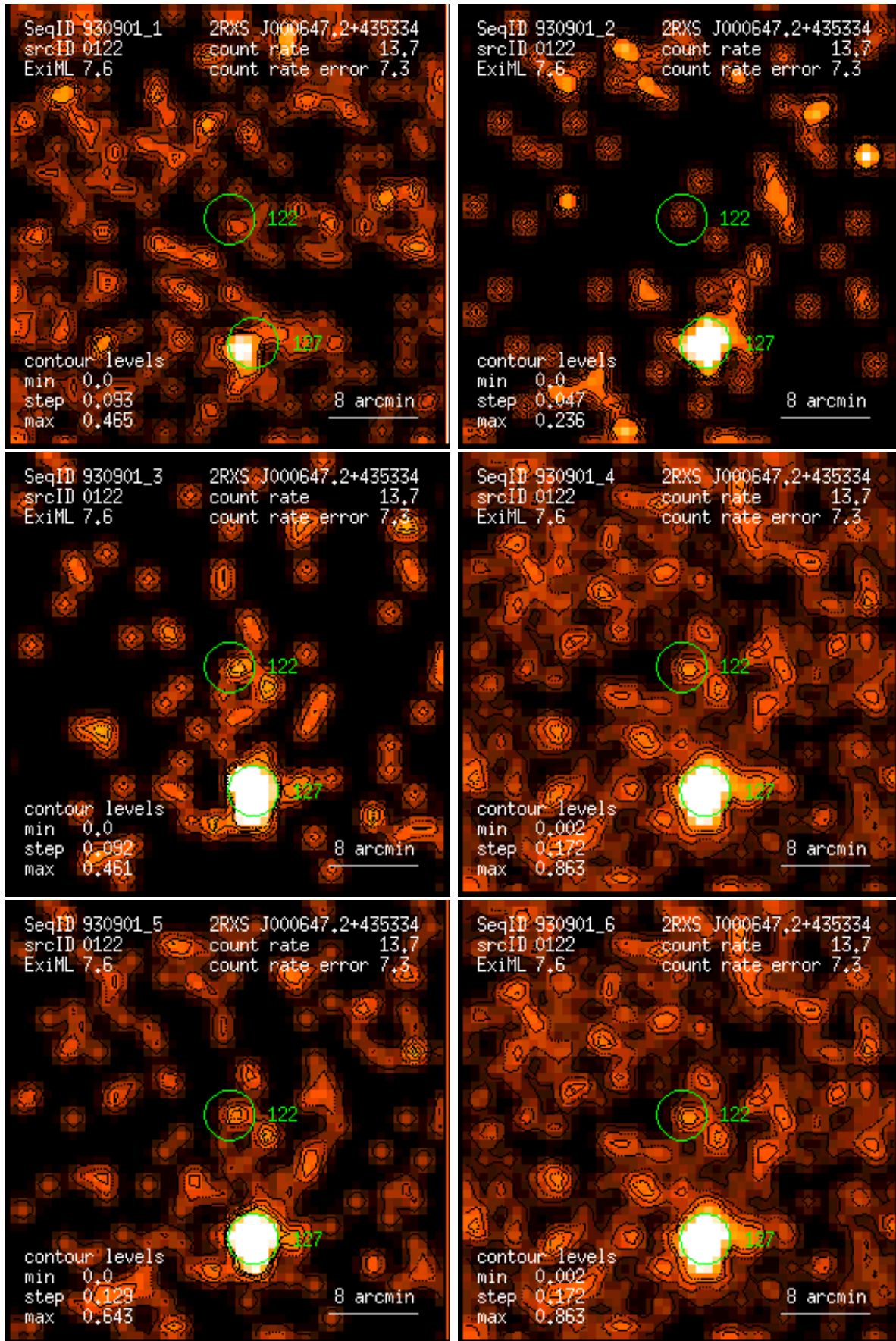
Figure 122: RASS 930901: detection 0122: band rate images, Gaussian filter: (1) PSPC channels 11 – 41, (2) 52 – 90, (3) 91 – 201, (4) 11 – 235, (5) 52 – 201, (6) 11 – 201. Broad band rates in counts/ks. Band rate contour levels in counts/ks/arcmin 2 .
