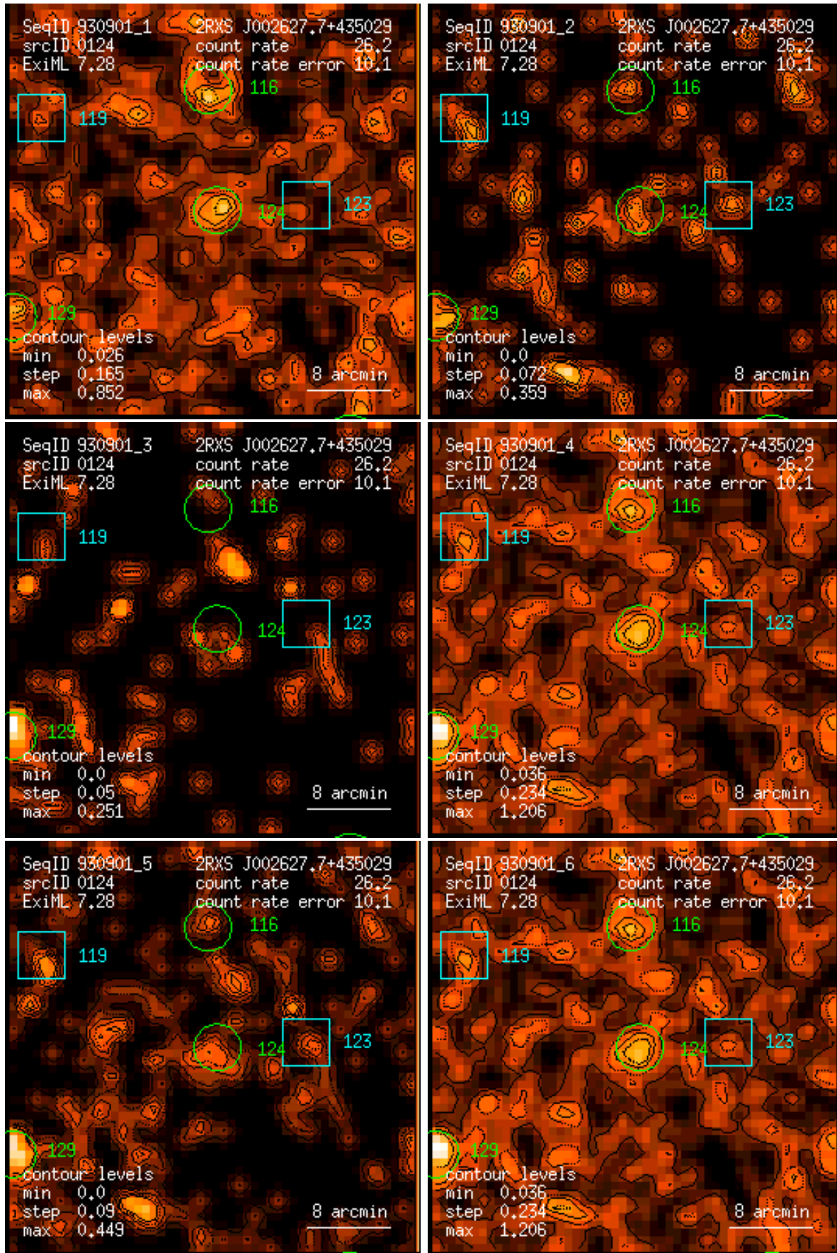
Figure 124: RASS 930901: detection 0124: band rate images, Gaussian filter: (1) PSPC channels 11 – 41, (2) 52 – 90, (3) 91 – 201, (4) 11 – 235, (5) 52 – 201, (6) 11 – 201. Broad band rates in counts/ks. Band rate contour levels in counts/ks/arcmin 2 .
