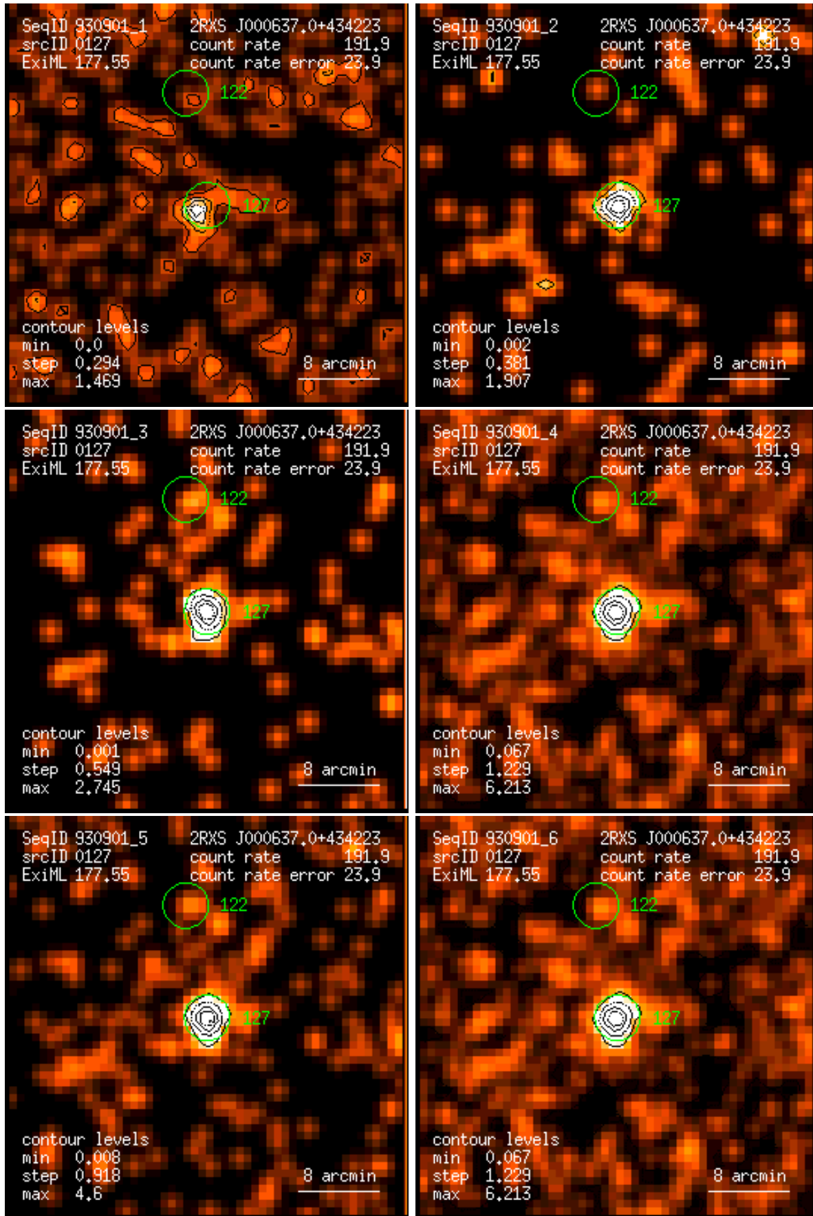
Figure 127: RASS 930901: detection 0127: band rate images, Gaussian filter: (1) PSPC channels 11 – 41, (2) 52 – 90, (3) 91 – 201, (4) 11 – 235, (5) 52 – 201, (6) 11 – 201. Broad band rates in counts/ks. Band rate contour levels in counts/ks/arcmin 2 .
