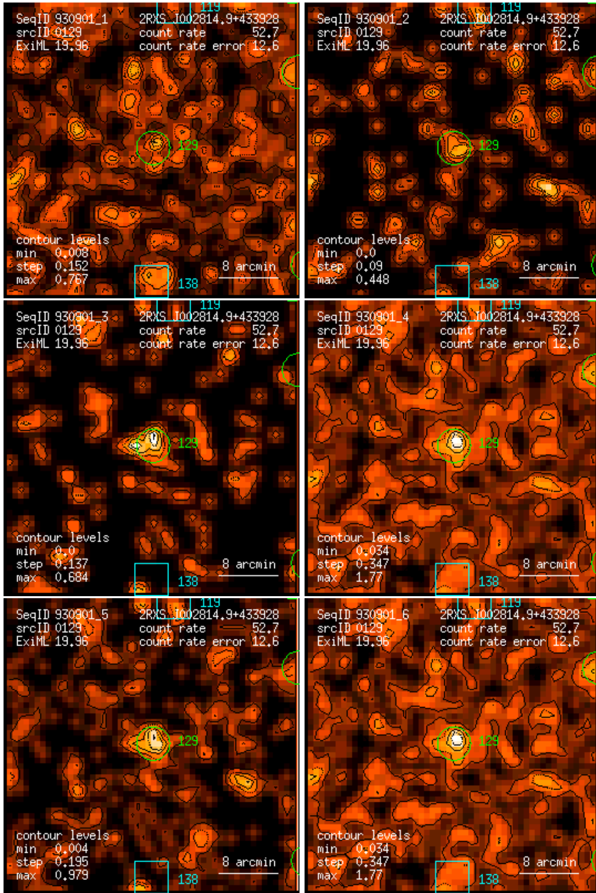
Figure 129: RASS 930901: detection 0129: band rate images, Gaussian filter: (1) PSPC channels 11 – 41, (2) 52 – 90, (3) 91 – 201, (4) 11 – 235, (5) 52 – 201, (6) 11 – 201. Broad band rates in counts/ks. Band rate contour levels in counts/ks/arcmin 2 .
