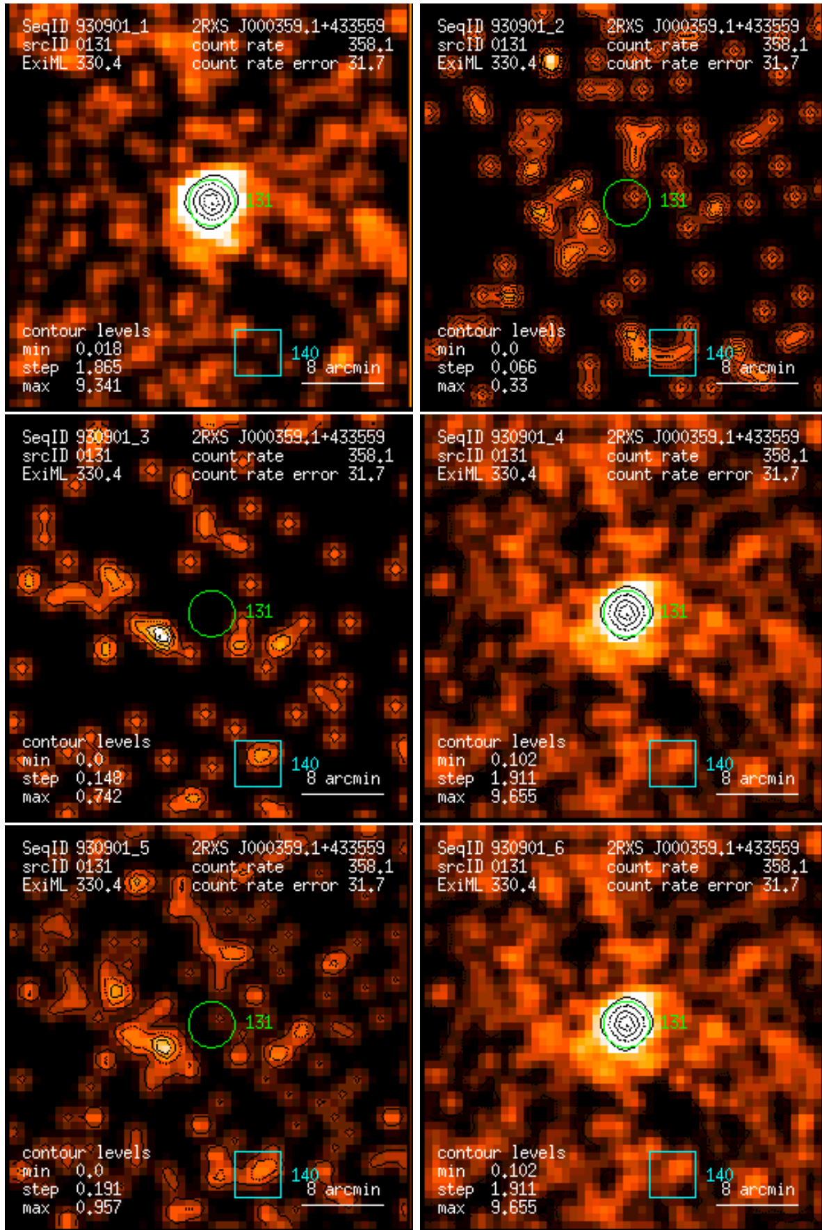
Figure 131: RASS 930901: detection 0131: band rate images, Gaussian filter: (1) PSPC channels 11 – 41, (2) 52 – 90, (3) 91 – 201, (4) 11 – 235, (5) 52 – 201, (6) 11 – 201. Broad band rates in counts/ks. Band rate contour levels in counts/ks/arcmin 2 .
