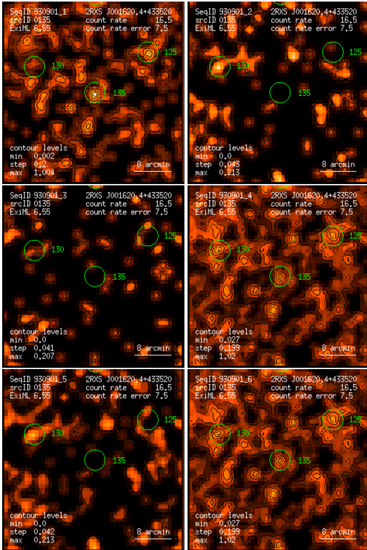
Figure 135: RASS 930901: detection 0135: band rate images, Gaussian filter: (1) PSPC channels 11 – 41, (2) 52 – 90, (3) 91 – 201, (4) 11 – 235, (5) 52 – 201, (6) 11 – 201. Broad band rates in counts/ks. Band rate contour levels in counts/ks/arcmin 2 .
