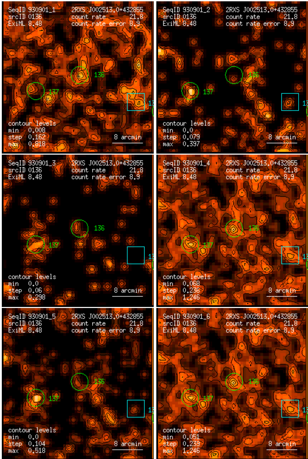
Figure 136: RASS 930901: detection 0136: band rate images, Gaussian filter: (1) PSPC channels 11 – 41, (2) 52 – 90, (3) 91 – 201, (4) 11 – 235, (5) 52 – 201, (6) 11 – 201. Broad band rates in counts/ks. Band rate contour levels in counts/ks/arcmin 2 .
