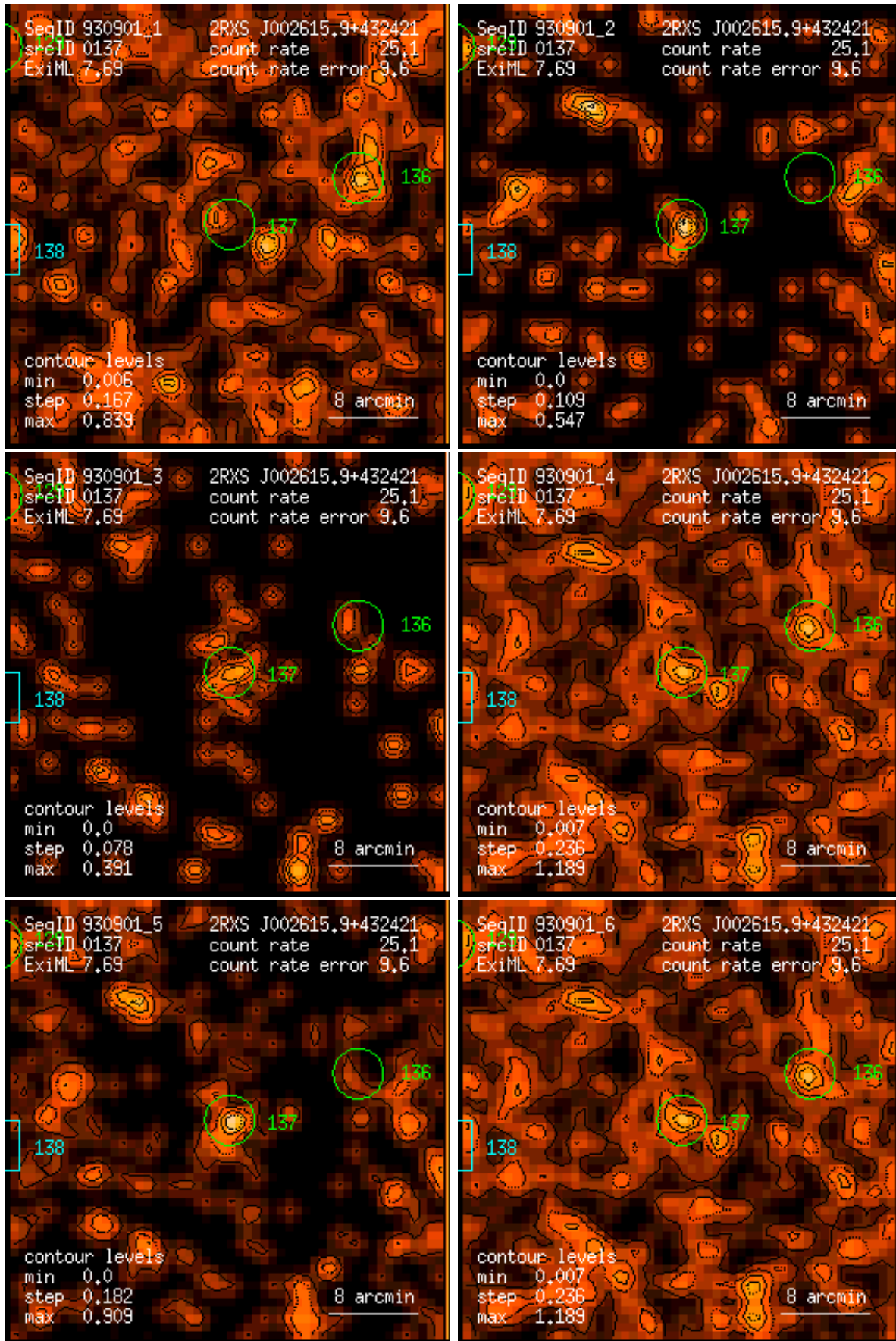
Figure 137: RASS 930901: detection 0137: band rate images, Gaussian filter: (1) PSPC channels 11 – 41, (2) 52 – 90, (3) 91 – 201, (4) 11 – 235, (5) 52 – 201, (6) 11 – 201. Broad band rates in counts/ks. Band rate contour levels in counts/ks/arcmin 2 .
