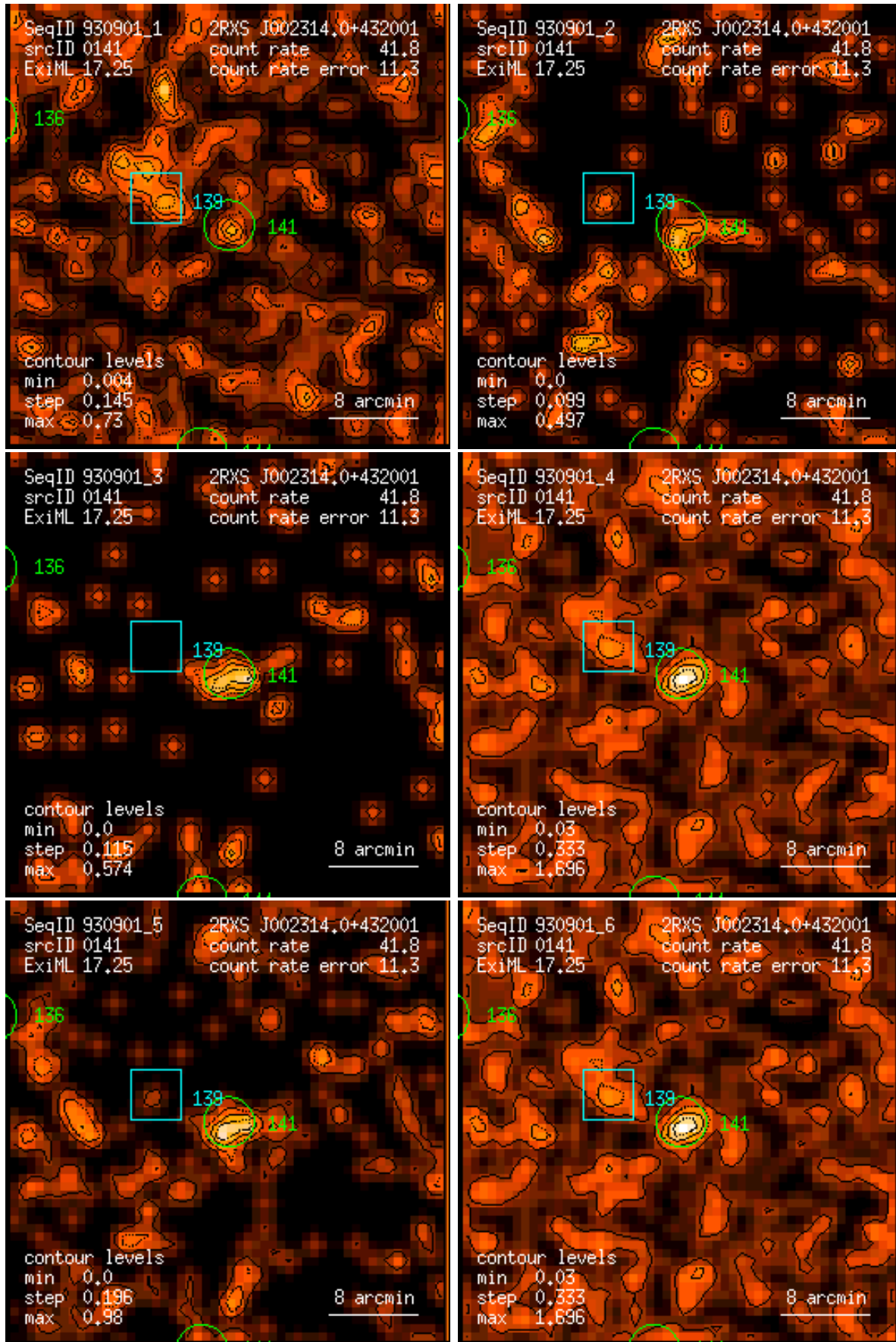
Figure 141: RASS 930901: detection 0141: band rate images, Gaussian filter: (1) PSPC channels 11 – 41, (2) 52 – 90, (3) 91 – 201, (4) 11 – 235, (5) 52 – 201, (6) 11 – 201. Broad band rates in counts/ks. Band rate contour levels in counts/ks/arcmin 2 .
