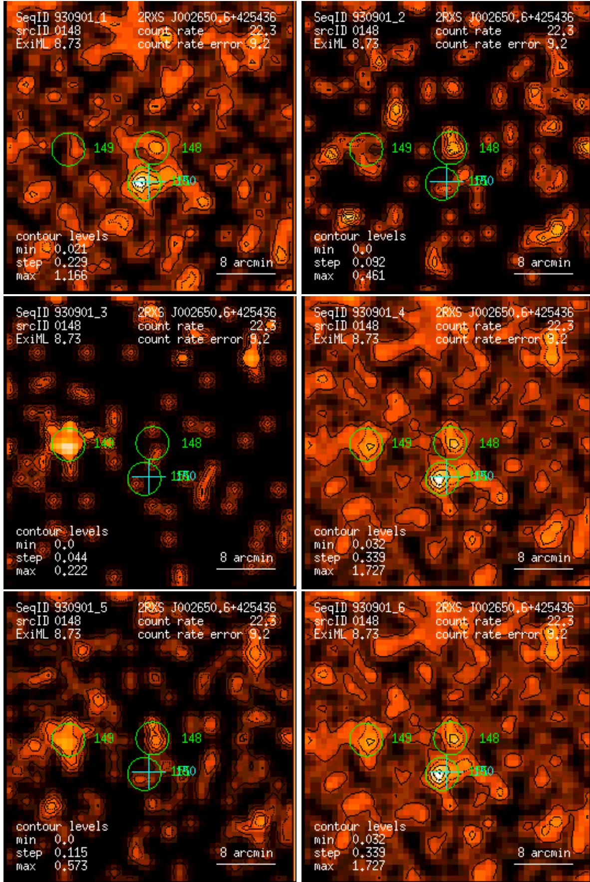
Figure 148: RASS 930901: detection 0148: band rate images, Gaussian filter: (1) PSPC channels 11 – 41, (2) 52 – 90, (3) 91 – 201, (4) 11 – 235, (5) 52 – 201, (6) 11 – 201. Broad band rates in counts/ks. Band rate contour levels in counts/ks/arcmin 2 .
