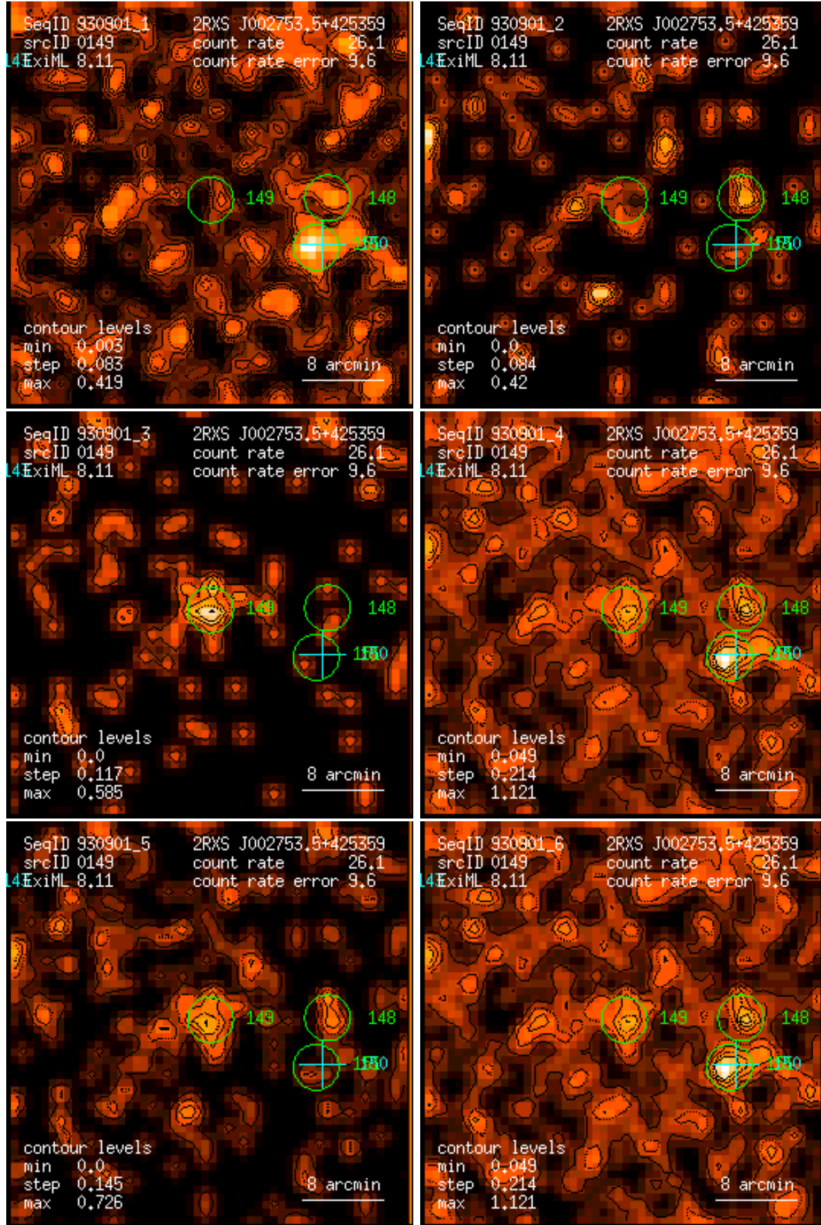
Figure 149: RASS 930901: detection 0149: band rate images, Gaussian filter: (1) PSPC channels 11 – 41, (2) 52 – 90, (3) 91 – 201, (4) 11 – 235, (5) 52 – 201, (6) 11 – 201. Broad band rates in counts/ks. Band rate contour levels in counts/ks/arcmin 2 .
