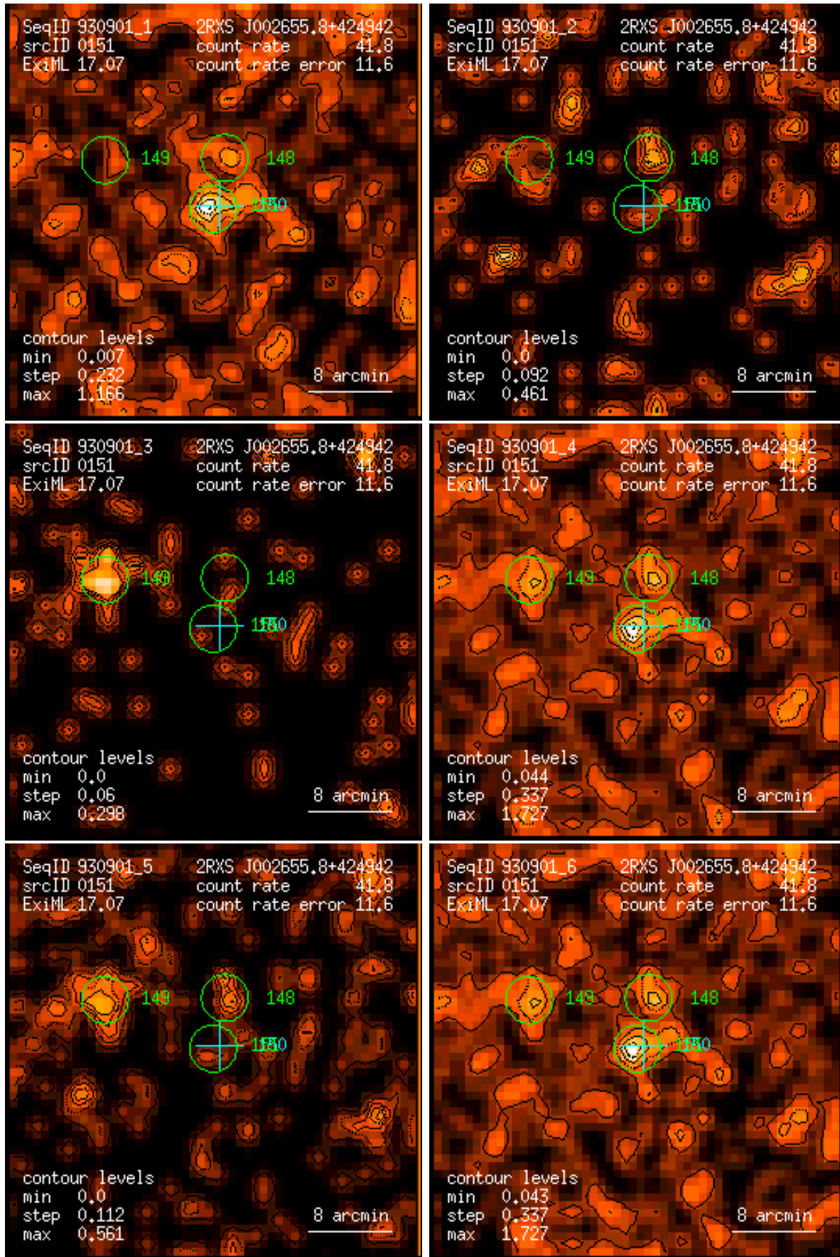
Figure 151: RASS 930901: detection 0151: band rate images, Gaussian filter: (1) PSPC channels 11 – 41, (2) 52 – 90, (3) 91 – 201, (4) 11 – 235, (5) 52 – 201, (6) 11 – 201. Broad band rates in counts/ks. Band rate contour levels in counts/ks/arcmin 2 .
