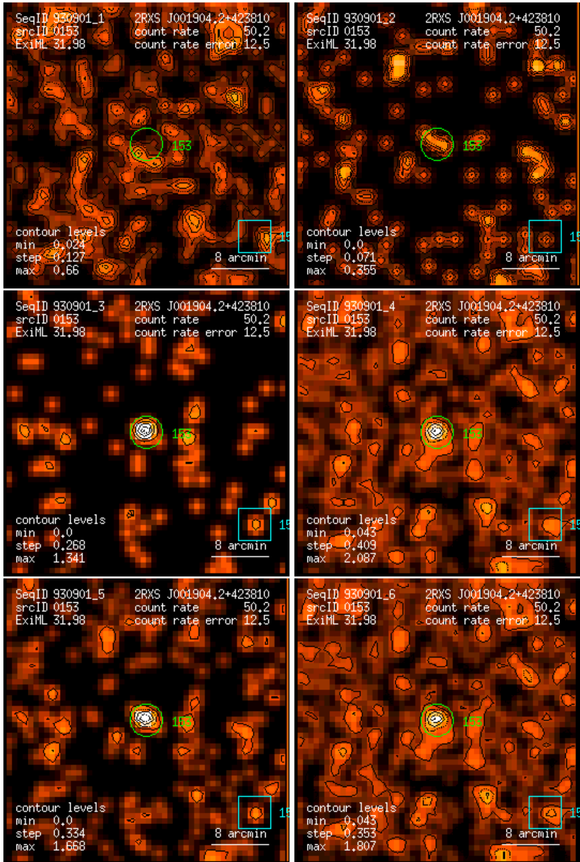
Figure 153: RASS 930901: detection 0153: band rate images, Gaussian filter: (1) PSPC channels 11 – 41, (2) 52 – 90, (3) 91 – 201, (4) 11 – 235, (5) 52 – 201, (6) 11 – 201. Broad band rates in counts/ks. Band rate contour levels in counts/ks/arcmin 2 .
