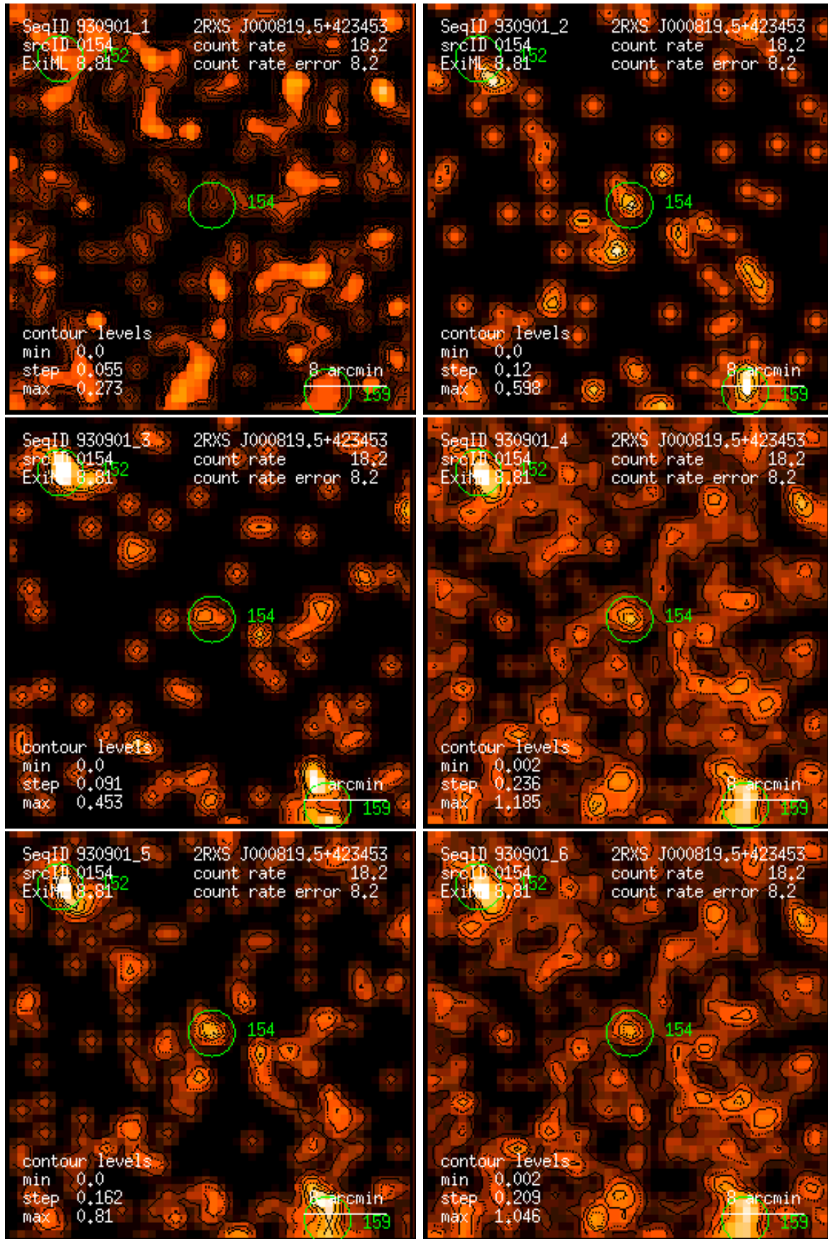
Figure 154: RASS 930901: detection 0154: band rate images, Gaussian filter: (1) PSPC channels 11 – 41, (2) 52 – 90, (3) 91 – 201, (4) 11 – 235, (5) 52 – 201, (6) 11 – 201. Broad band rates in counts/ks. Band rate contour levels in counts/ks/arcmin 2 .
