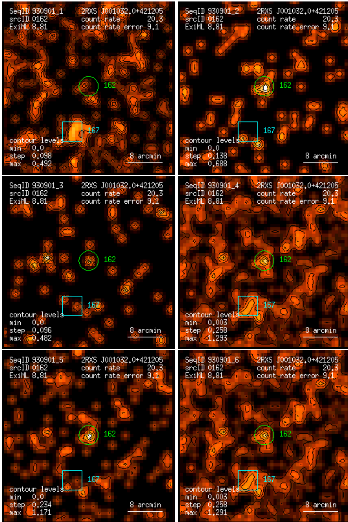
Figure 162: RASS 930901: detection 0162: band rate images, Gaussian filter: (1) PSPC channels 11 – 41, (2) 52 – 90, (3) 91 – 201, (4) 11 – 235, (5) 52 – 201, (6) 11 – 201. Broad band rates in counts/ks. Band rate contour levels in counts/ks/arcmin 2 .
