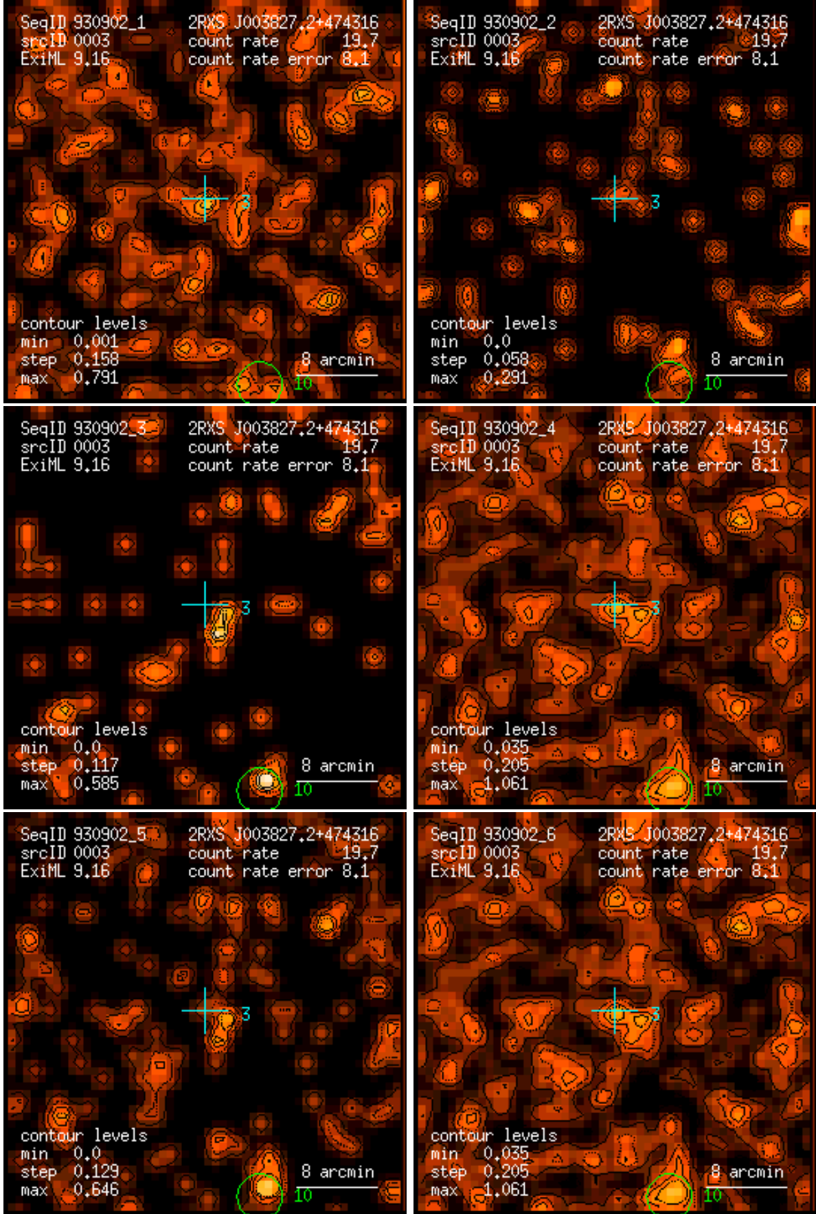
Figure 3: RASS 930902: detection 0003: band rate images, Gaussian filter: (1) PSPC channels 11 – 41, (2) 52 – 90, (3) 91 – 201, (4) 11 – 235, (5) 52 – 201, (6) 11 – 201. Broad band rates in counts/ks. Band rate contour levels in counts/ks/arcmin 2 .
