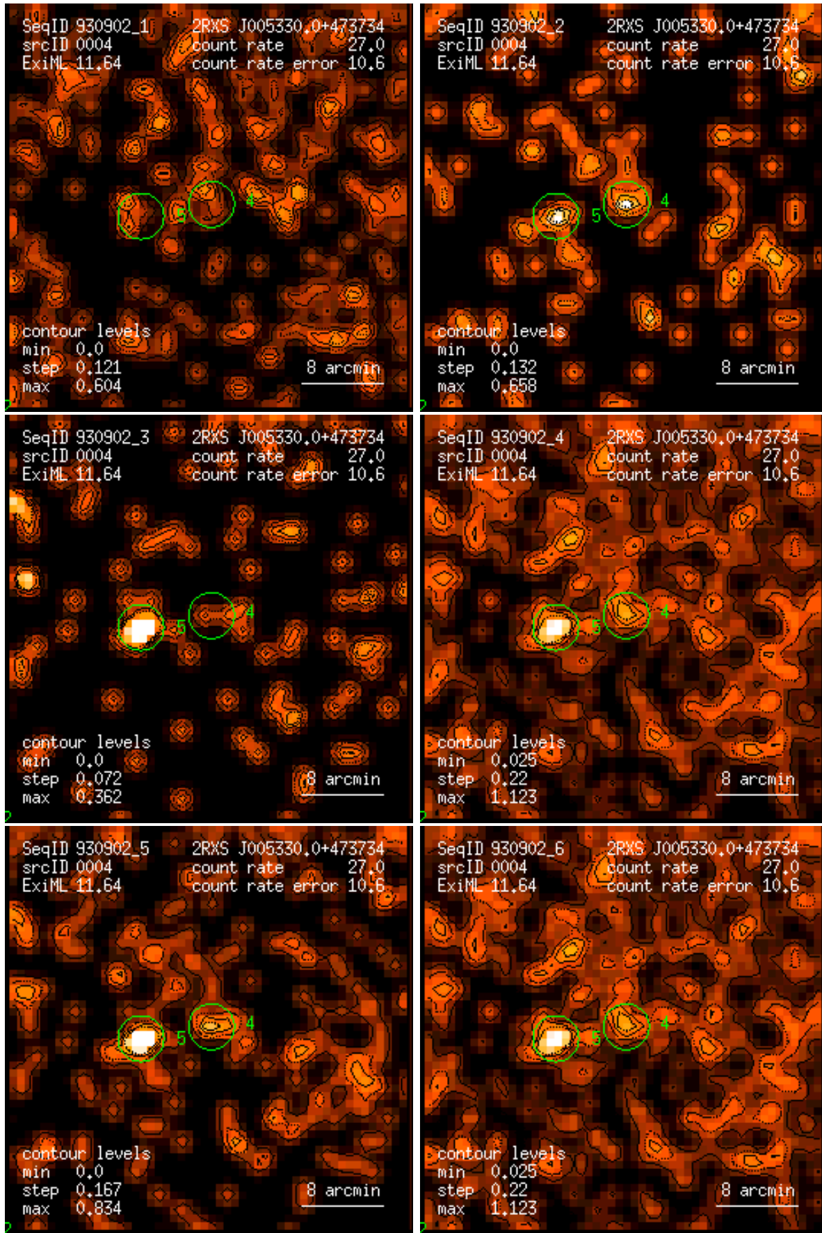
Figure 4: RASS 930902: detection 0004: band rate images, Gaussian filter: (1) PSPC channels 11 – 41, (2) 52 – 90, (3) 91 – 201, (4) 11 – 235, (5) 52 – 201, (6) 11 – 201. Broad band rates in counts/ks. Band rate contour levels in counts/ks/arcmin 2 .
