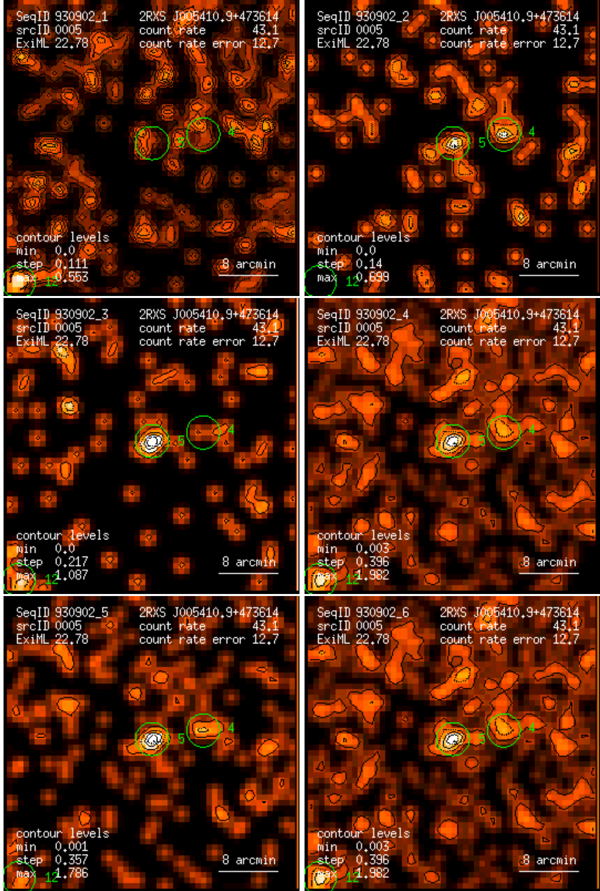
Figure 5: RASS 930902: detection 0005: band rate images, Gaussian filter: (1) PSPC channels 11 – 41, (2) 52 – 90, (3) 91 – 201, (4) 11 – 235, (5) 52 – 201, (6) 11 – 201. Broad band rates in counts/ks. Band rate contour levels in counts/ks/arcmin 2 .
