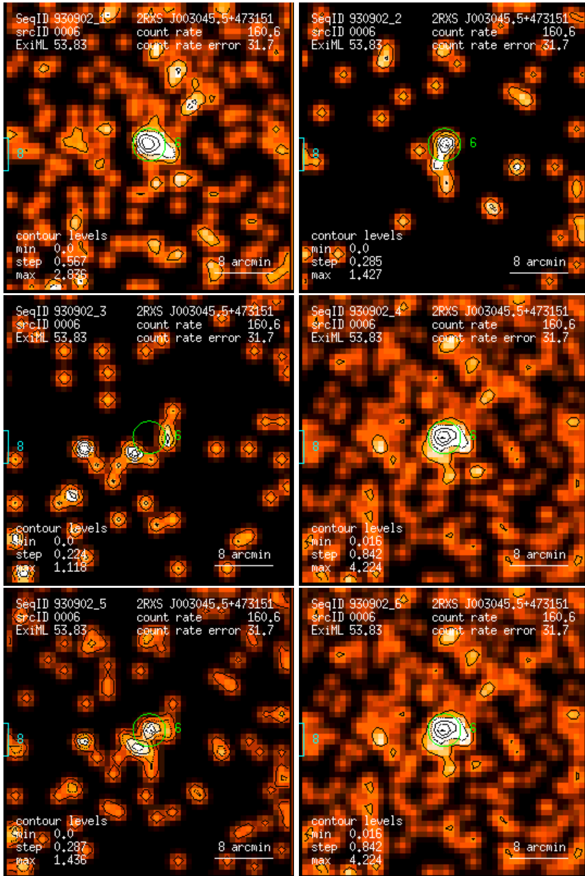
Figure 6: RASS 930902: detection 0006: band rate images, Gaussian filter: (1) PSPC channels 11 – 41, (2) 52 – 90, (3) 91 – 201, (4) 11 – 235, (5) 52 – 201, (6) 11 – 201. Broad band rates in counts/ks. Band rate contour levels in counts/ks/arcmin 2 .
