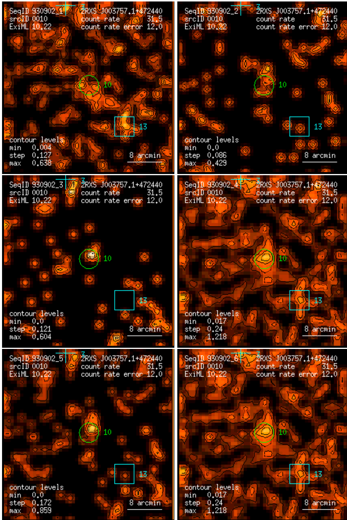
Figure 10: RASS 930902: detection 0010: band rate images, Gaussian filter: (1) PSPC channels 11 – 41, (2) 52 – 90, (3) 91 – 201, (4) 11 – 235, (5) 52 – 201, (6) 11 – 201. Broad band rates in counts/ks. Band rate contour levels in counts/ks/arcmin 2 .
