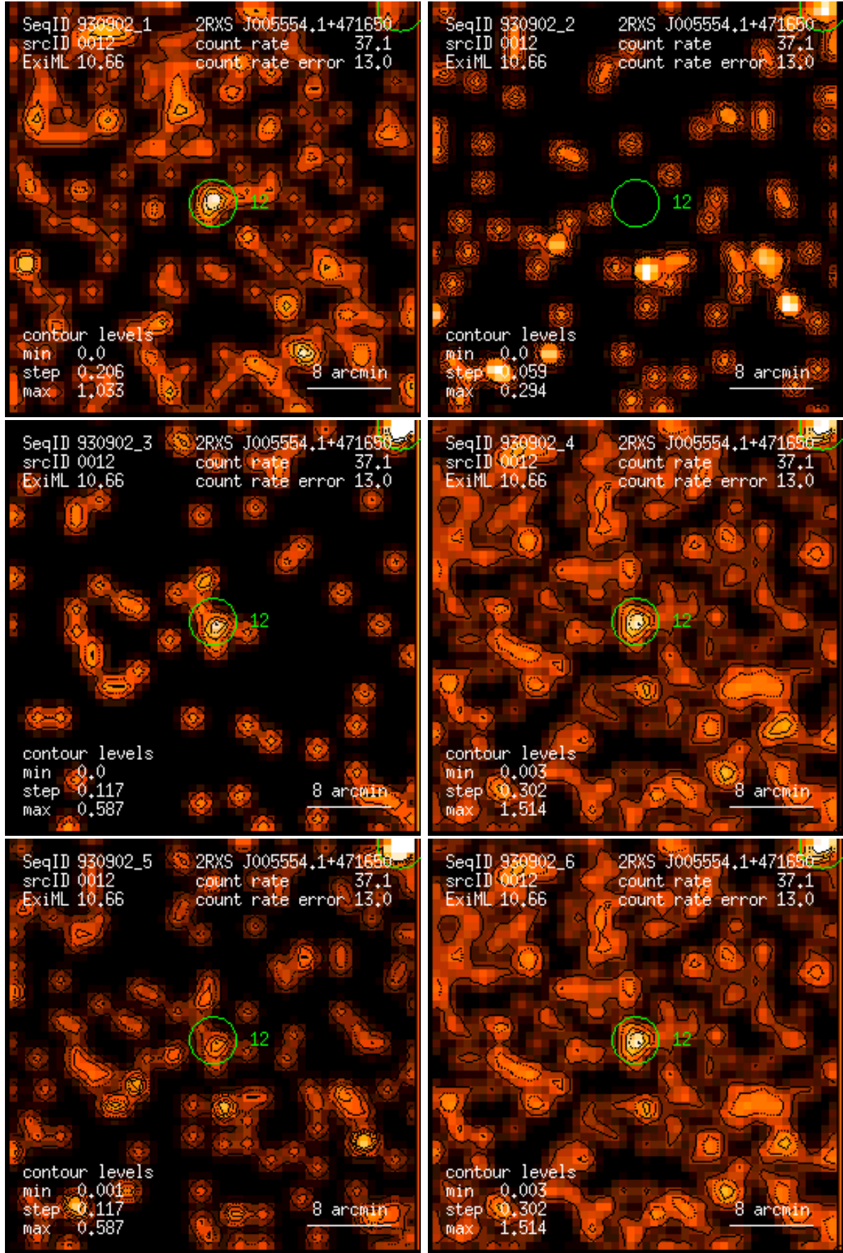
Figure 12: RASS 930902: detection 0012: band rate images, Gaussian filter: (1) PSPC channels 11 – 41, (2) 52 – 90, (3) 91 – 201, (4) 11 – 235, (5) 52 – 201, (6) 11 – 201. Broad band rates in counts/ks. Band rate contour levels in counts/ks/arcmin 2 .
