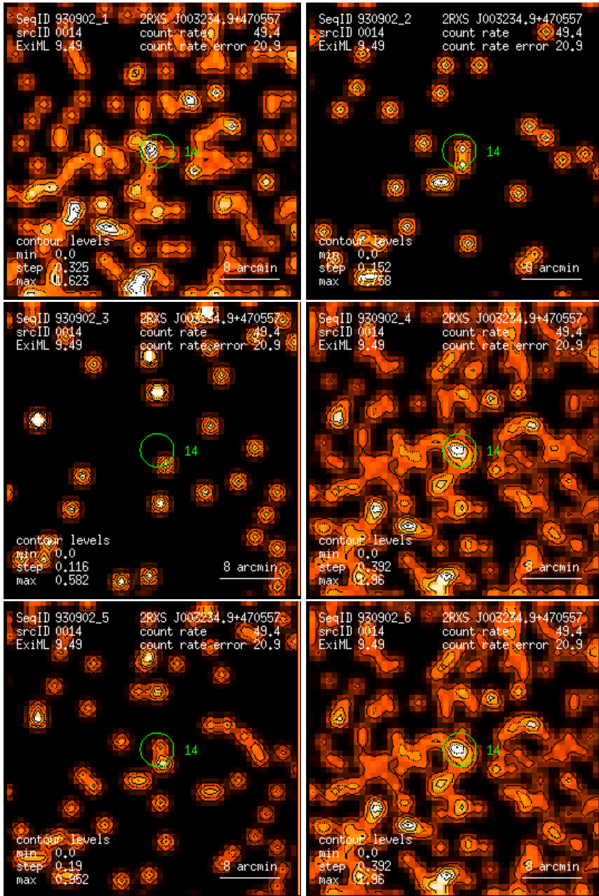
Figure 14: RASS 930902: detection 0014: band rate images, Gaussian filter: (1) PSPC channels 11 – 41, (2) 52 – 90, (3) 91 – 201, (4) 11 – 235, (5) 52 – 201, (6) 11 – 201. Broad band rates in counts/ks. Band rate contour levels in counts/ks/arcmin 2 .
