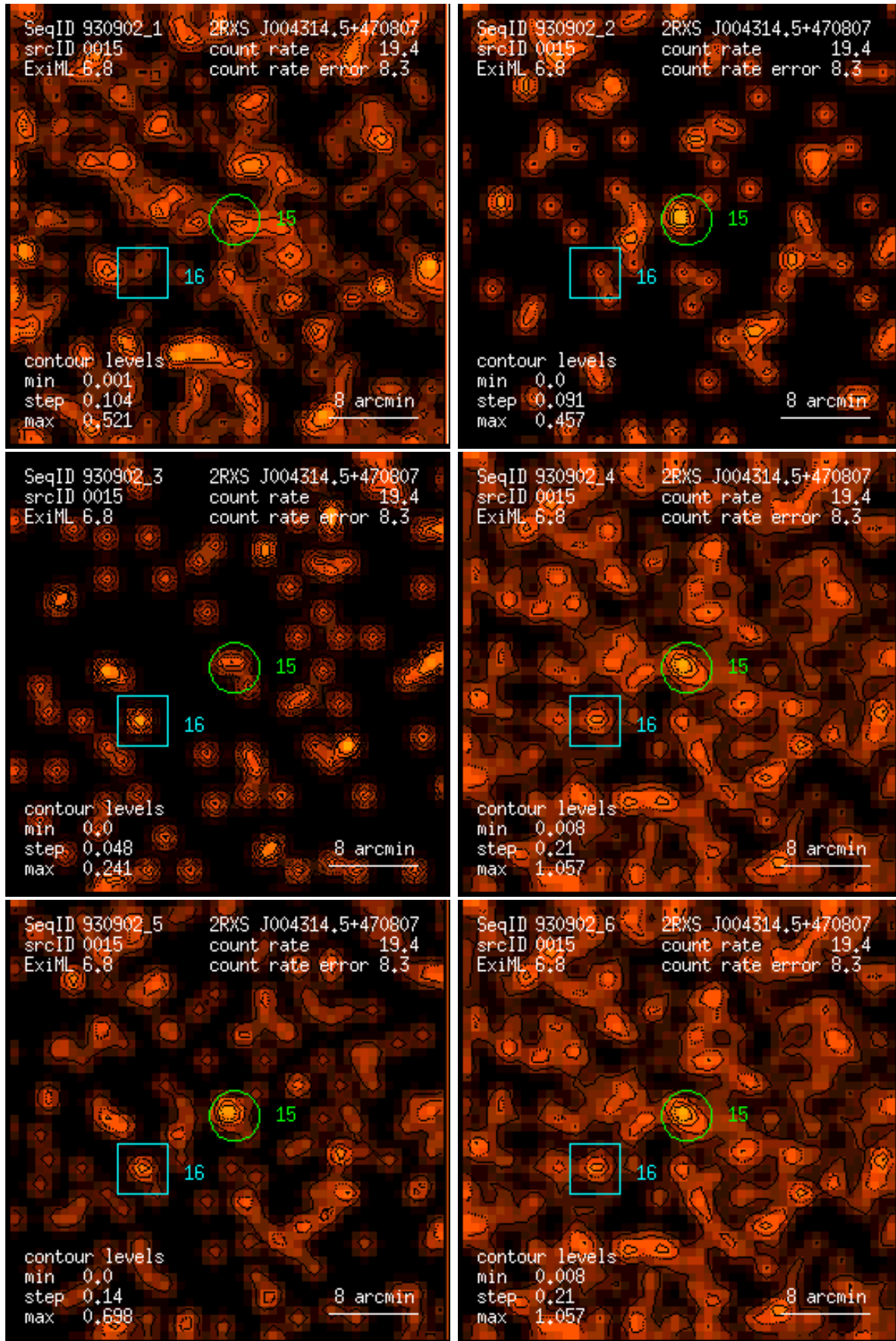
Figure 15: RASS 930902: detection 0015: band rate images, Gaussian filter: (1) PSPC channels 11 – 41, (2) 52 – 90, (3) 91 – 201, (4) 11 – 235, (5) 52 – 201, (6) 11 – 201. Broad band rates in counts/ks. Band rate contour levels in counts/ks/arcmin 2 .
