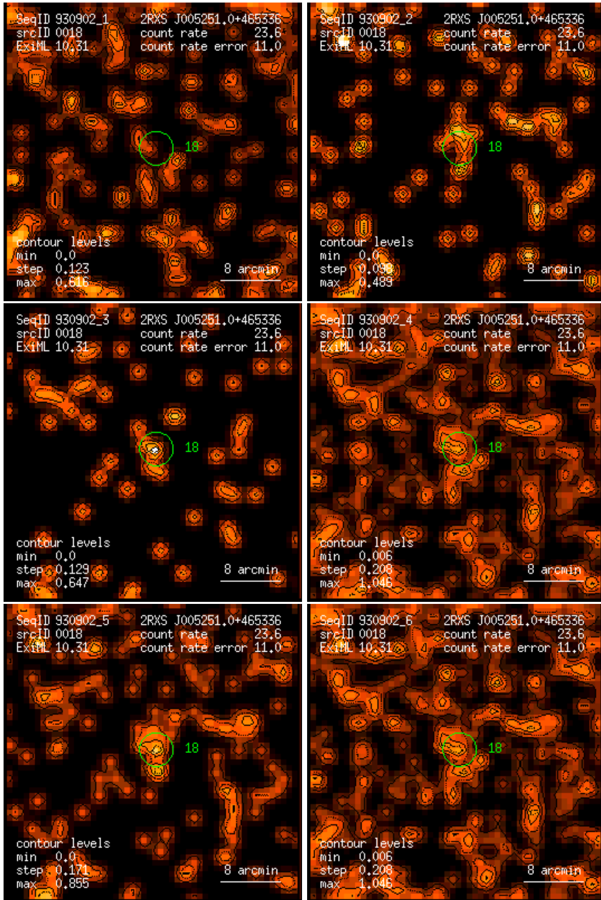
Figure 18: RASS 930902: detection 0018: band rate images, Gaussian filter: (1) PSPC channels 11 – 41, (2) 52 – 90, (3) 91 – 201, (4) 11 – 235, (5) 52 – 201, (6) 11 – 201. Broad band rates in counts/ks. Band rate contour levels in counts/ks/arcmin 2 .
