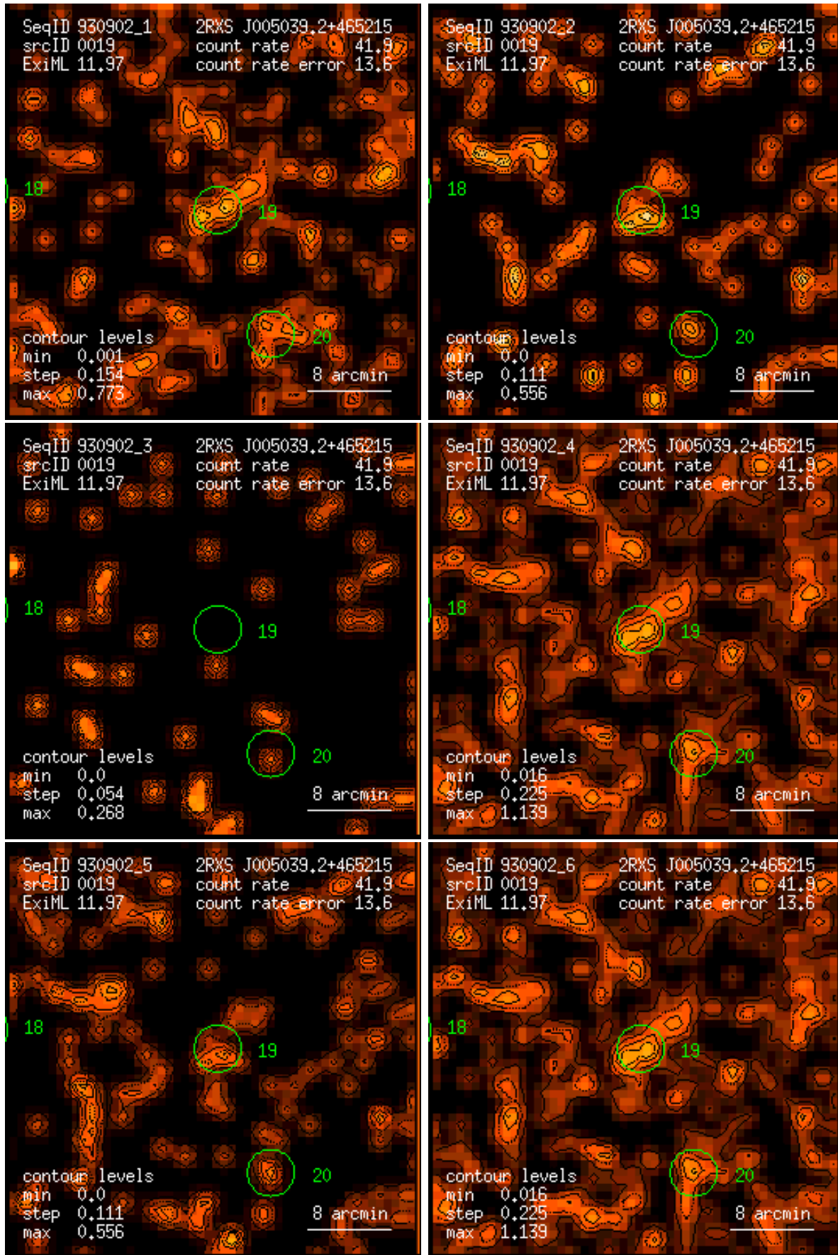
Figure 19: RASS 930902: detection 0019: band rate images, Gaussian filter: (1) PSPC channels 11 – 41, (2) 52 – 90, (3) 91 – 201, (4) 11 – 235, (5) 52 – 201, (6) 11 – 201. Broad band rates in counts/ks. Band rate contour levels in counts/ks/arcmin 2 .
