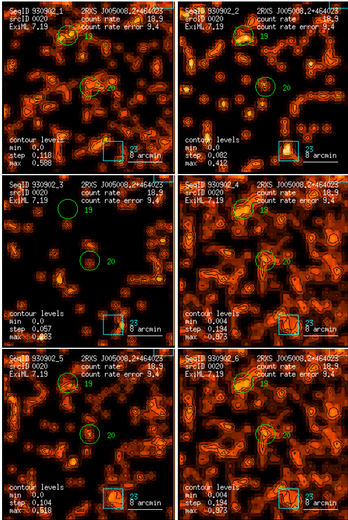
Figure 20: RASS 930902: detection 0020: band rate images, Gaussian filter: (1) PSPC channels 11 – 41, (2) 52 – 90, (3) 91 – 201, (4) 11 – 235, (5) 52 – 201, (6) 11 – 201. Broad band rates in counts/ks. Band rate contour levels in counts/ks/arcmin 2 .
