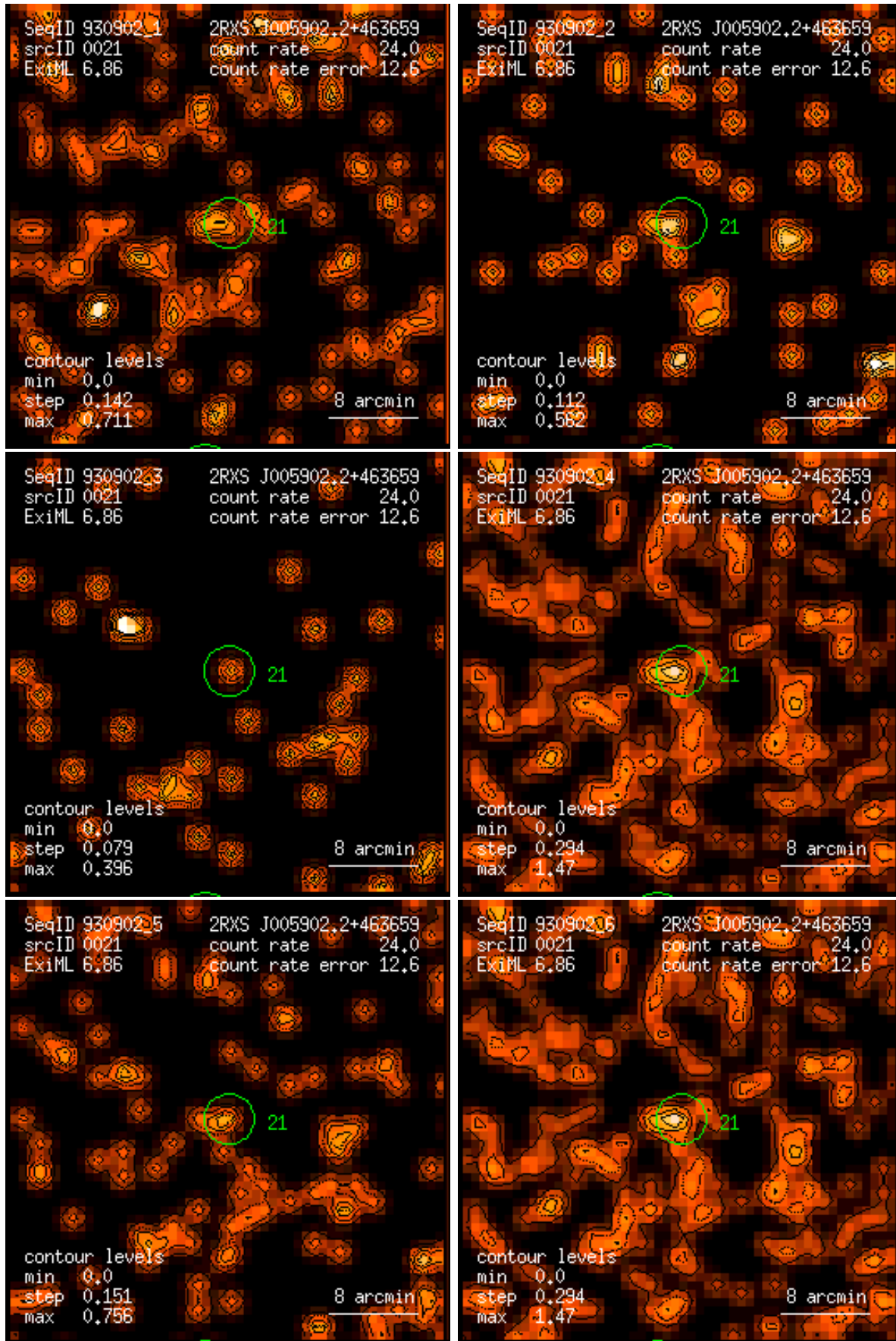
Figure 21: RASS 930902: detection 0021: band rate images, Gaussian filter: (1) PSPC channels 11 – 41, (2) 52 – 90, (3) 91 – 201, (4) 11 – 235, (5) 52 – 201, (6) 11 – 201. Broad band rates in counts/ks. Band rate contour levels in counts/ks/arcmin 2 .
