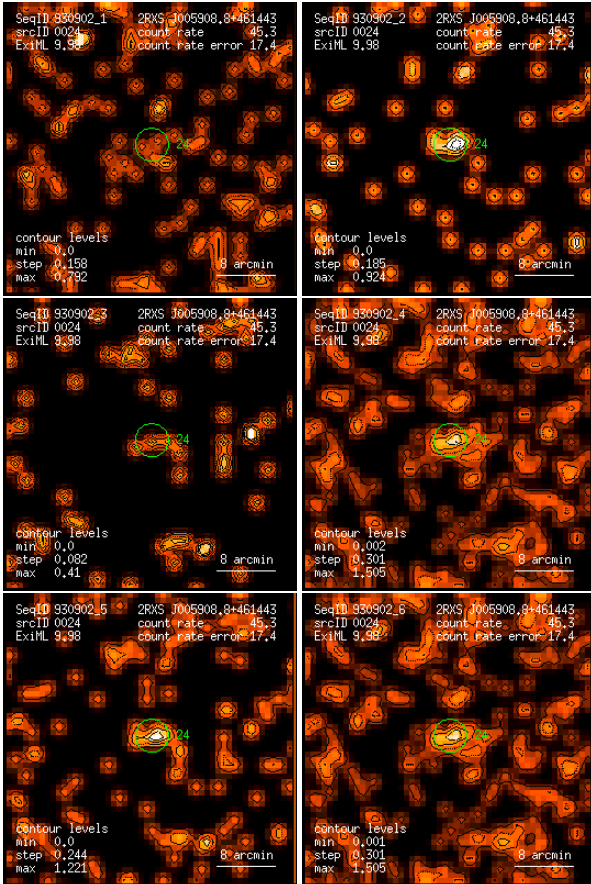
Figure 24: RASS 930902: detection 0024: band rate images, Gaussian filter: (1) PSPC channels 11 – 41, (2) 52 – 90, (3) 91 – 201, (4) 11 – 235, (5) 52 – 201, (6) 11 – 201. Broad band rates in counts/ks. Band rate contour levels in counts/ks/arcmin 2 .
